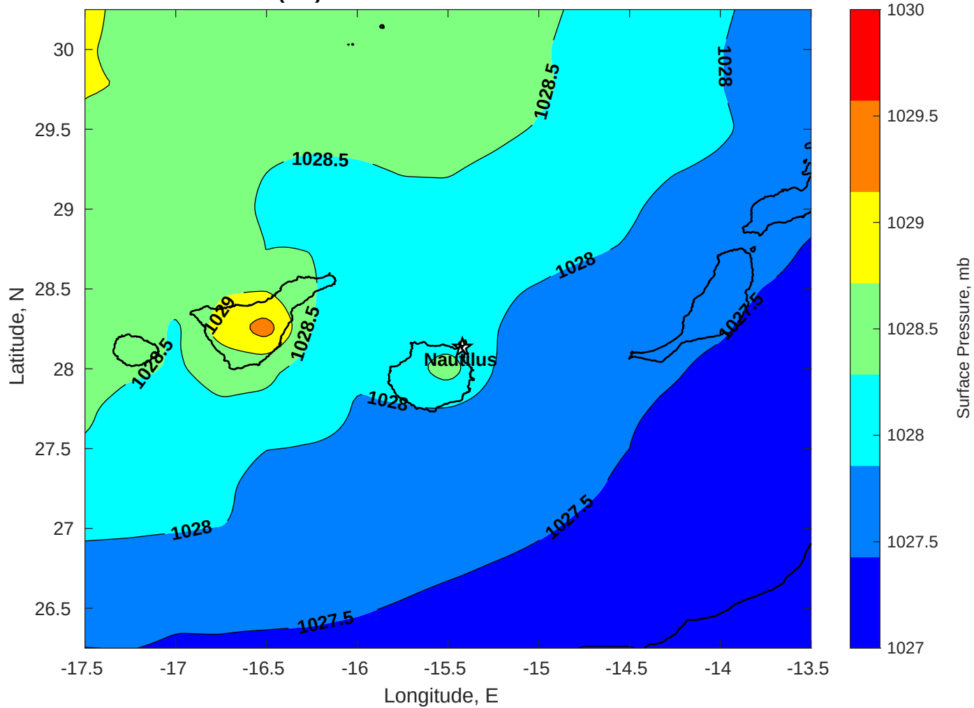
Surface Pressure (mb) for Nautilus at 25-Jan-2026 00:00:00
