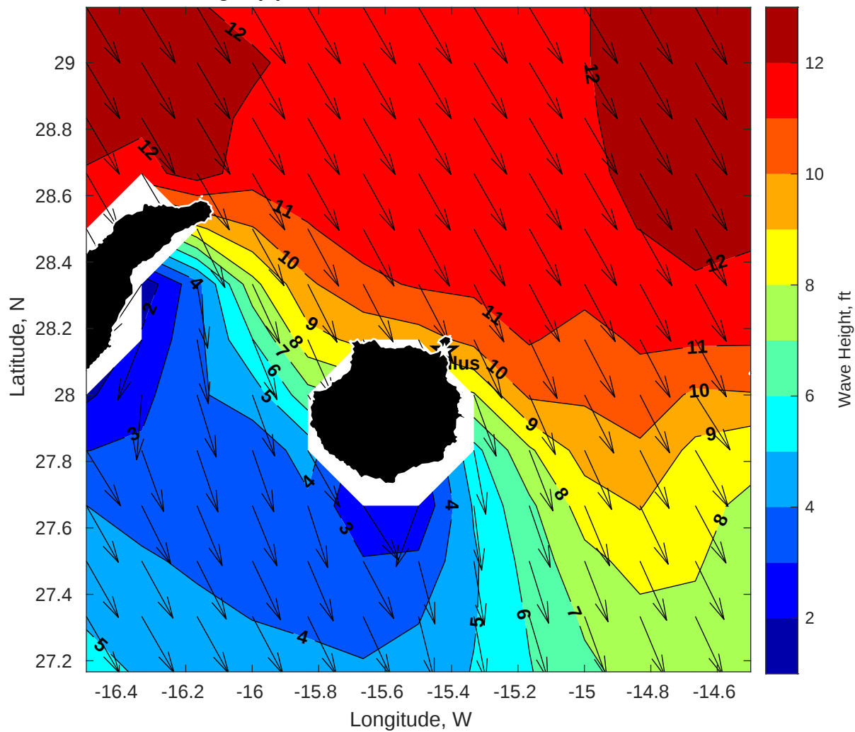
GFS Wave Height (ft) for Nautilus at 25-Jan-2026 09:00:00
