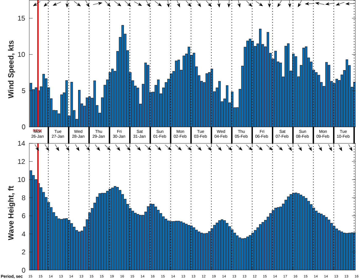
Wind & Wave Forecast for Nautilus from 25-Jan-2026 02:00:00 to 10-Feb-2026 02:00:00
