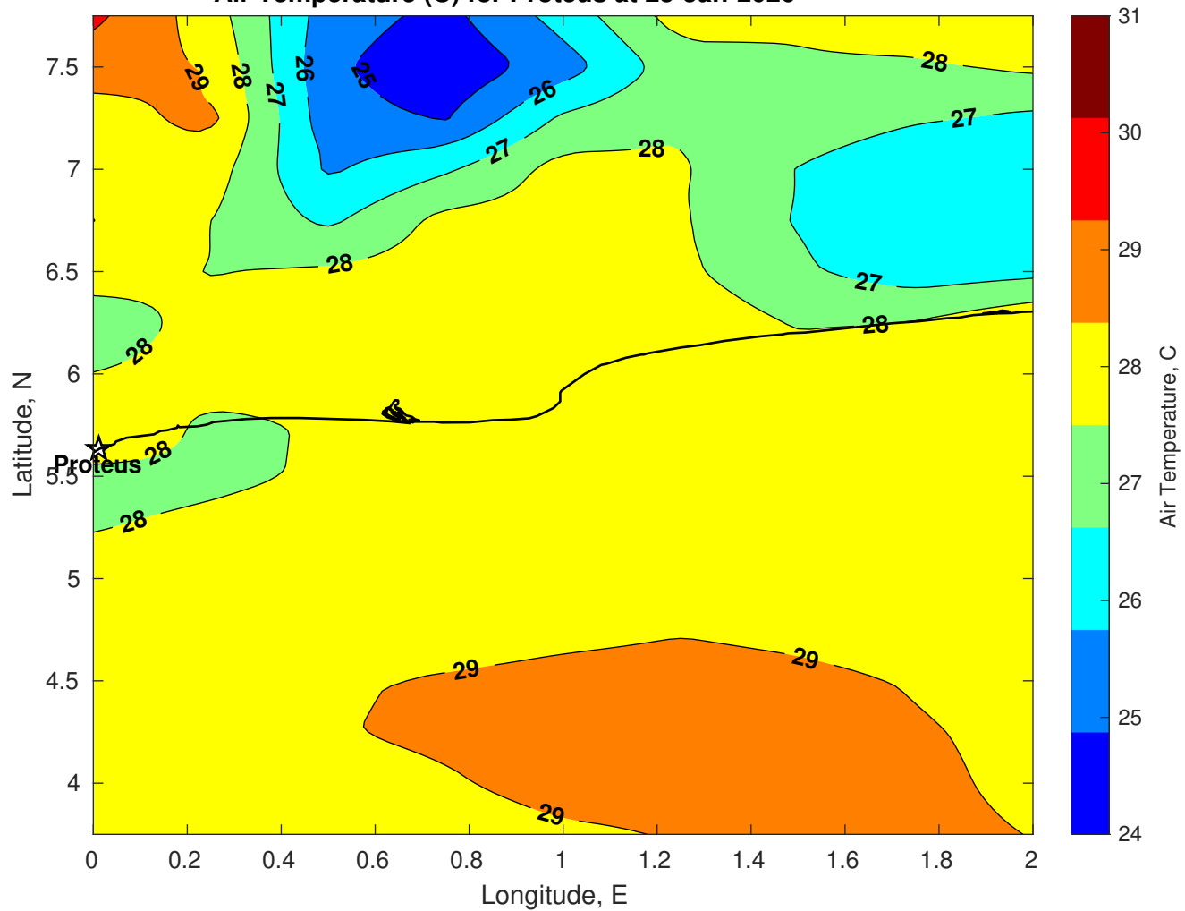
Air Temperature (C) for Proteus at 25-Jan-2026
