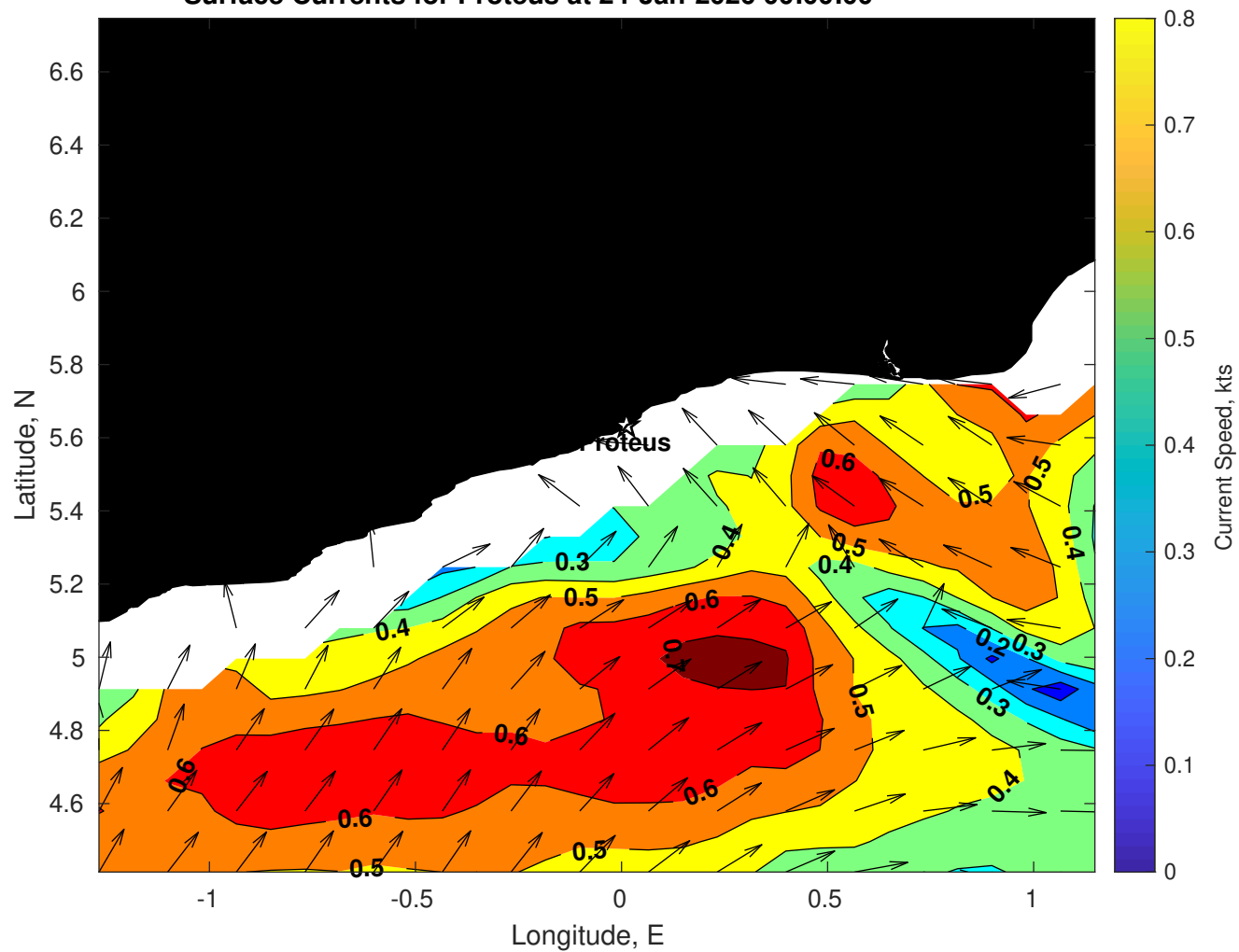
Surface Currents for Proteus at 24-Jan-2026 00:00:00
