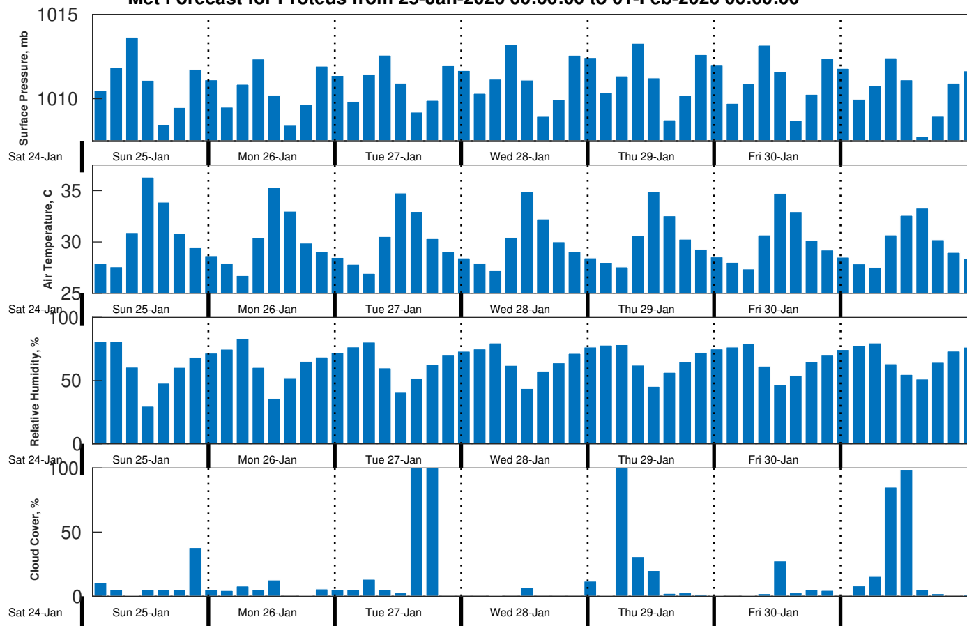
Met Forecast for Proteus from 25-Jan-2026 00:00:00 to 01-Feb-2026 00:00:00
