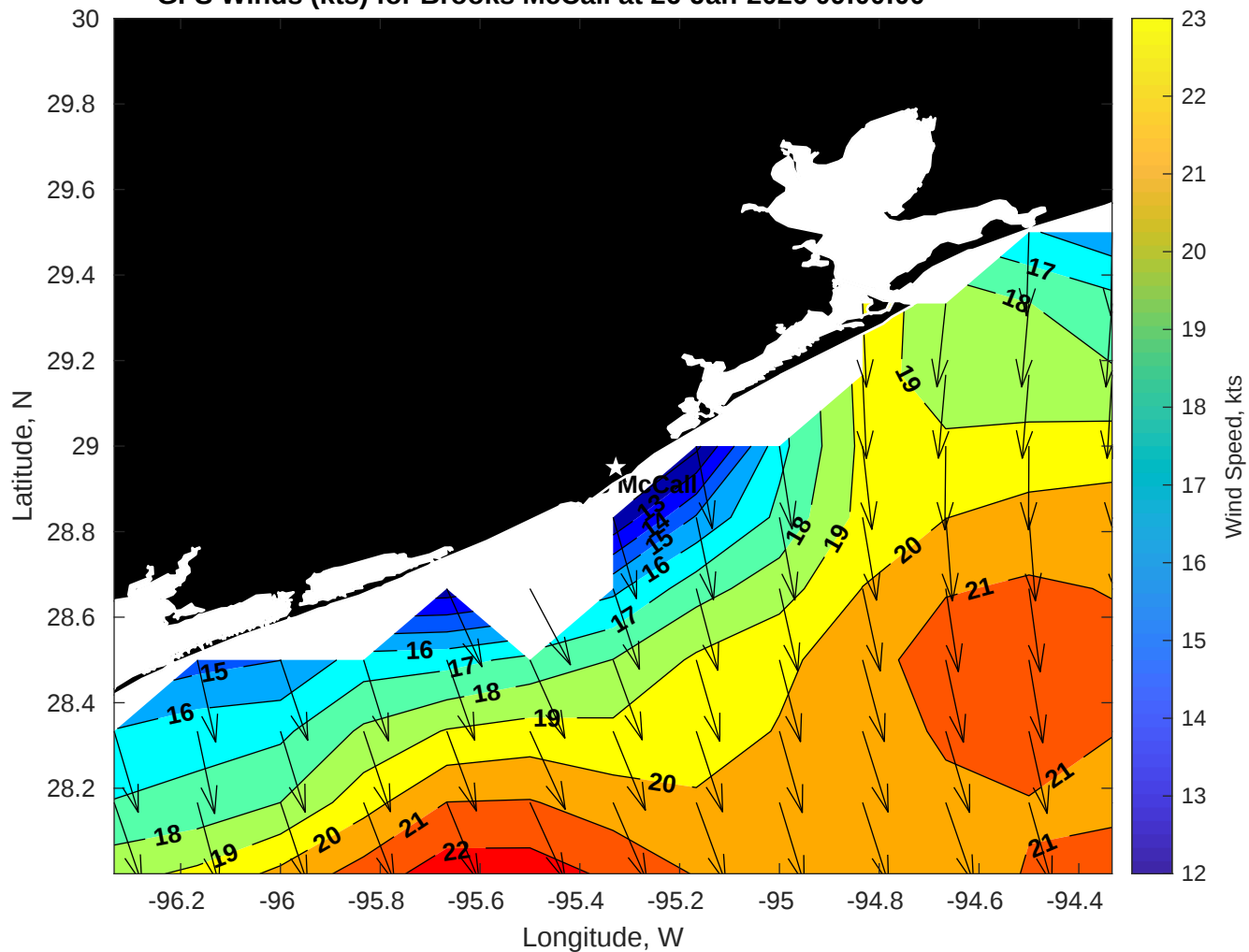
GFS Winds (kts) for Brooks McCall at 26-Jan-2026 09:00:00
