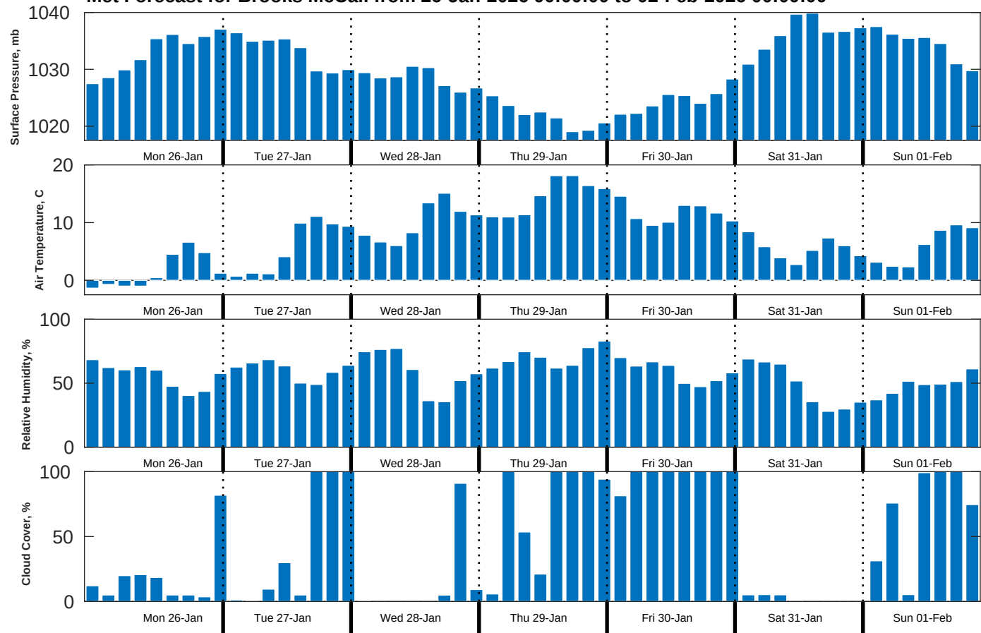
Met Forecast for Brooks McCall from 26-Jan-2026 00:00:00 to 02-Feb-2026 00:00:00
