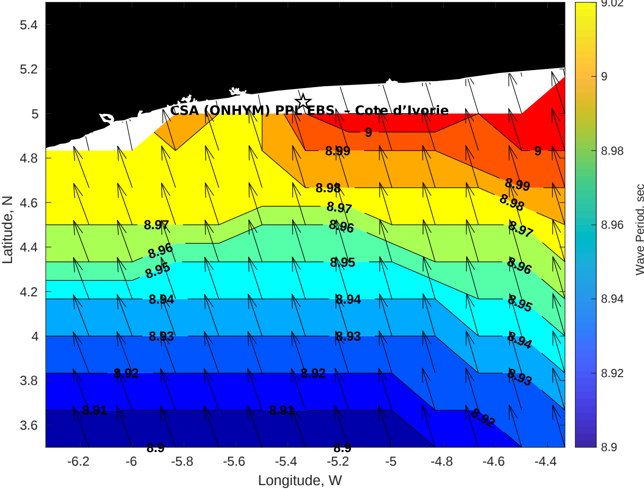
GFS Wave Period (sec) for CSA (ONHYM) PPL EBS - Cote d'Ivoire at 26-Jan-2026 09:00:00
