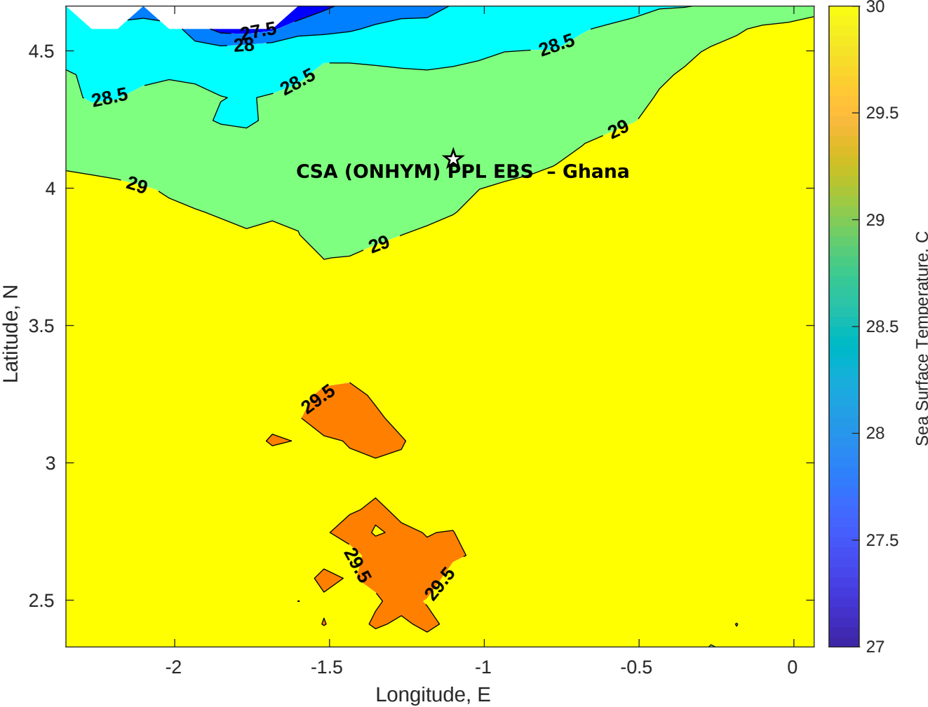
SST for CSA (ONHYM) PPL EBS - Ghana at 25-Jan-2026 00:00:00
