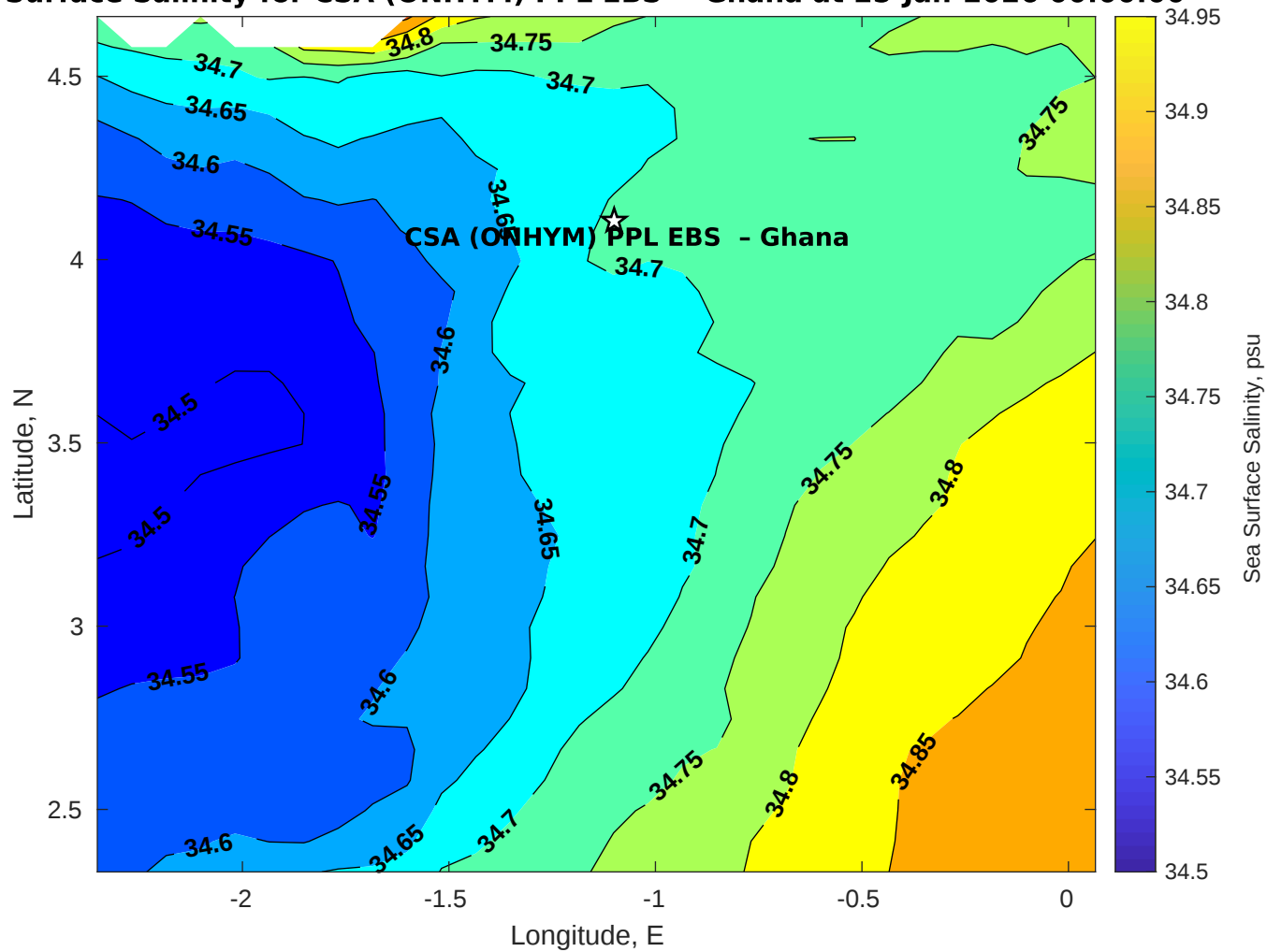
Surface Salinity for CSA (ONHYM) PPL EBS - Ghana at 25-Jan-2026 00:00:00
