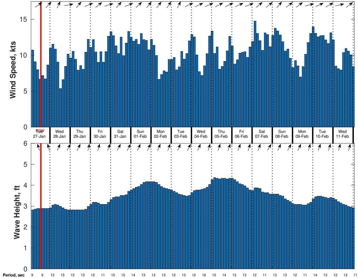
Wind & Wave Forecast for CSA (ONHYM) PPL EBS - Ghana from 26-Jan-2026 02:00:00 to 11-Feb-2026 02:00:00
