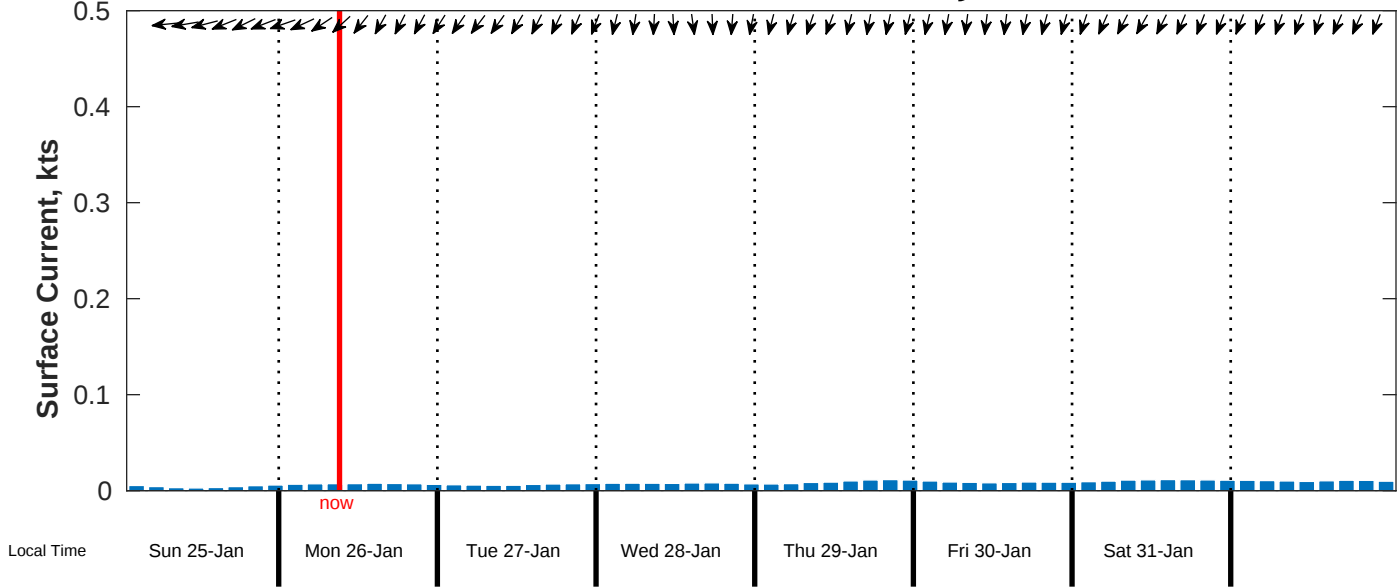
Surface Current Forecast for CSA (ONHYM) PPL EBS - Ghana from 25-Jan-2026 00:00:00 to 02-Feb-2026 00:00:00
