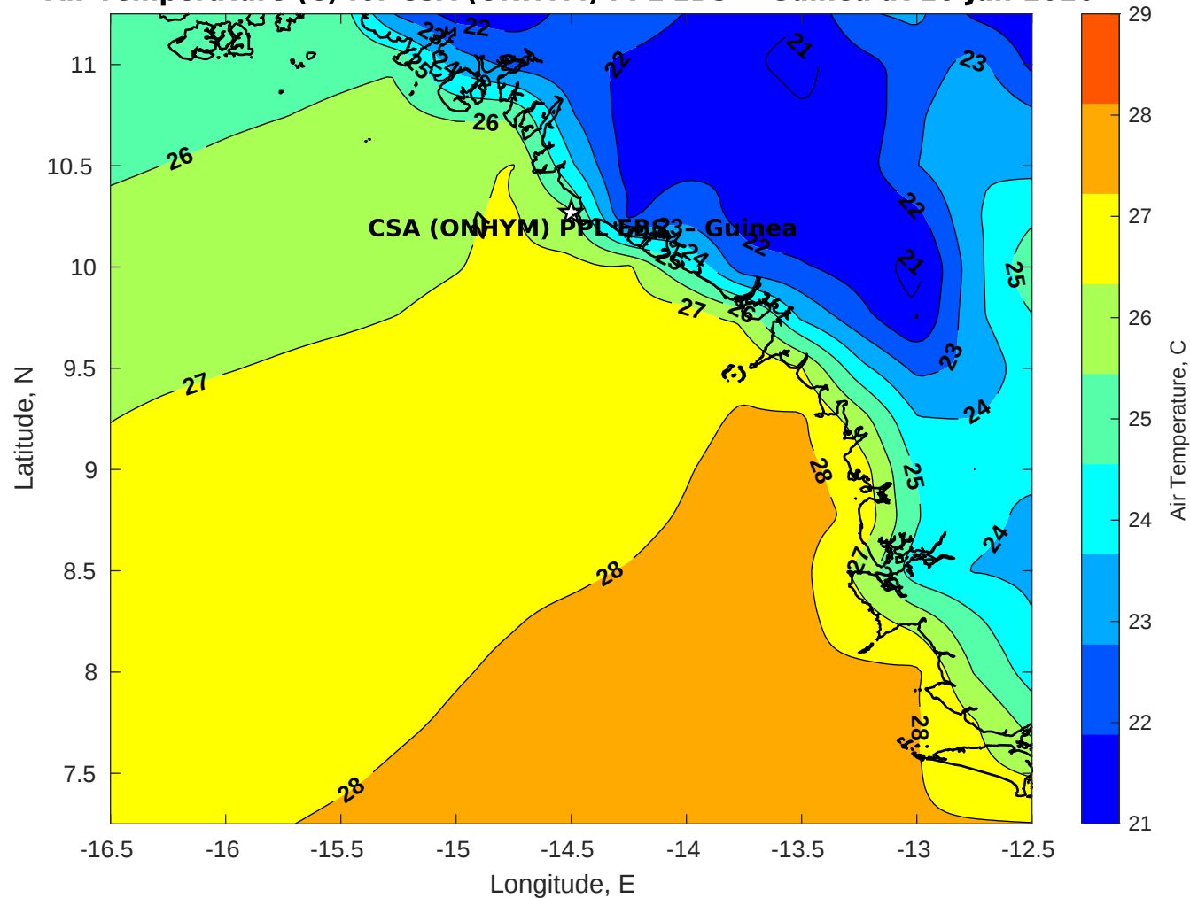
Air Temperature (C) for CSA (ONHYM) PPL EBS - Guinea at 26-Jan-2026
