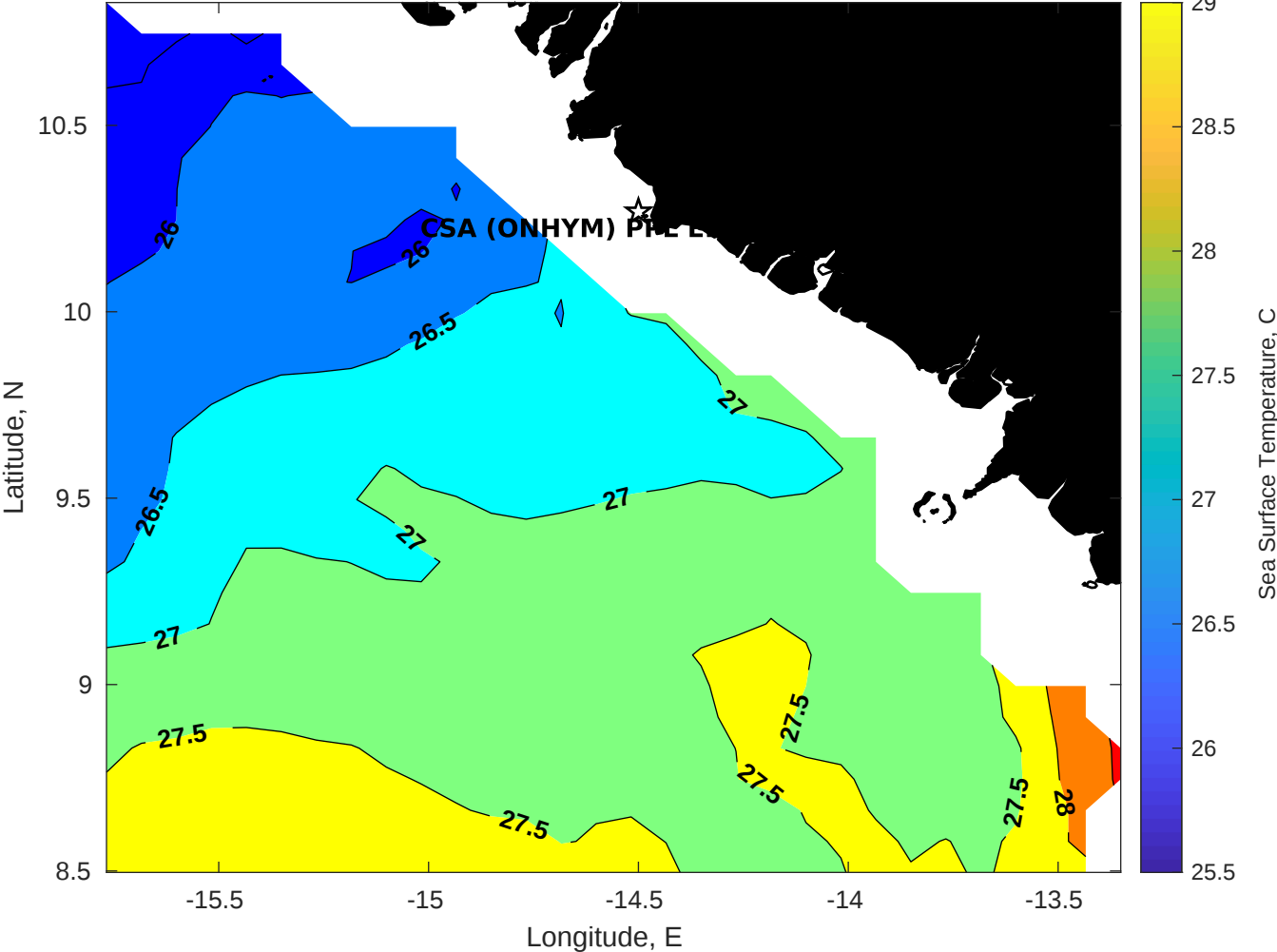
SST for CSA (ONHYM) PPL EBS - Guinea at 25-Jan-2026 00:00:00
