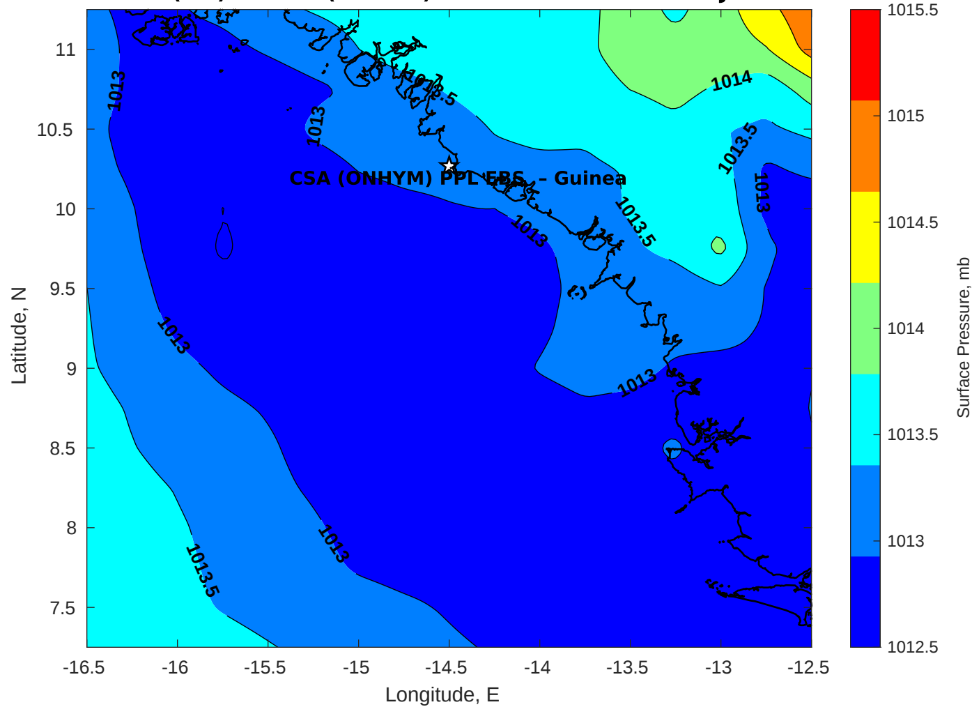
Surface Pressure (mb) for CSA (ONHYM) PPL EBS - Guinea at 28-Jan-2026 00:00:00
