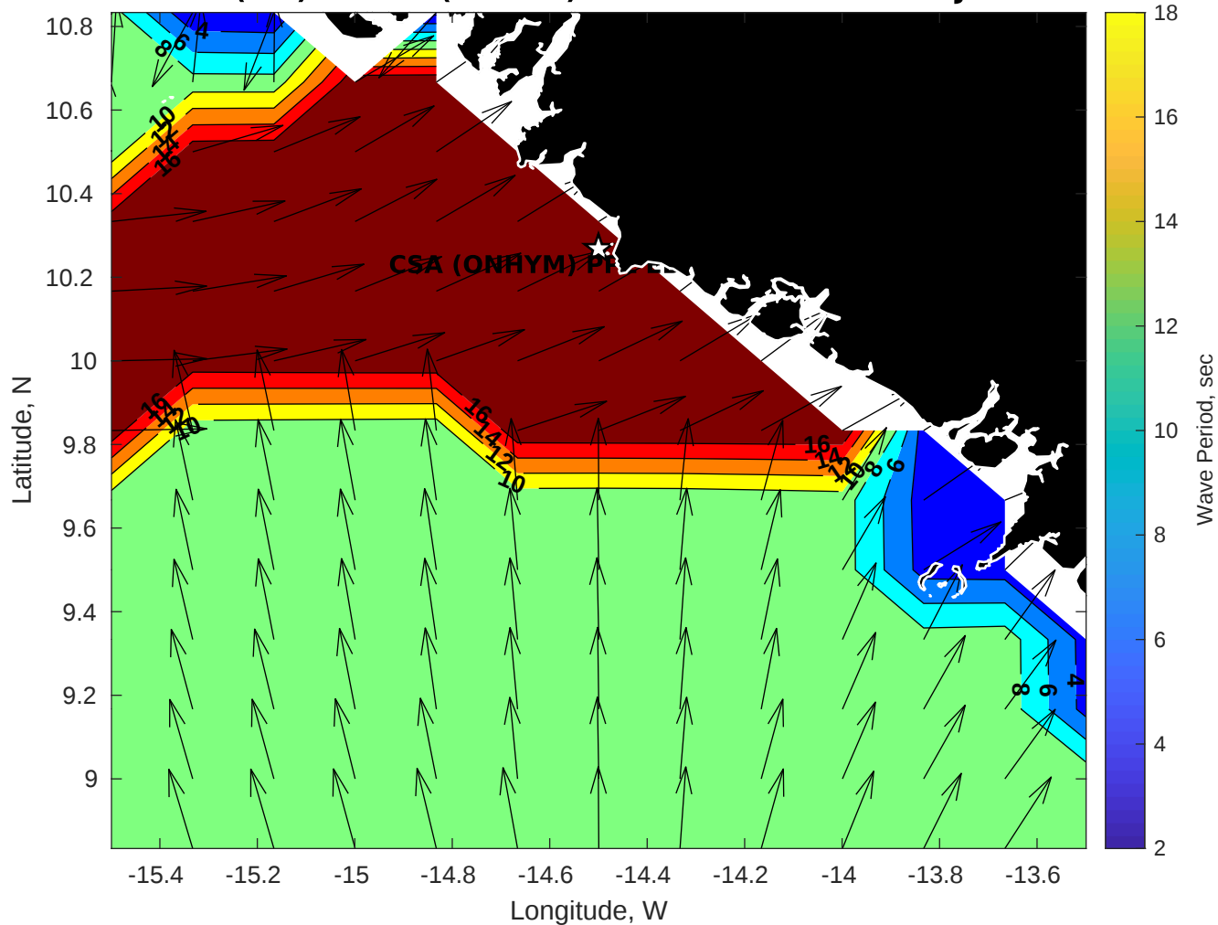
GFS Wave Period (sec) for CSA (ONHYM) PPL EBS - Guinea at 26-Jan-2026 09:00:00
