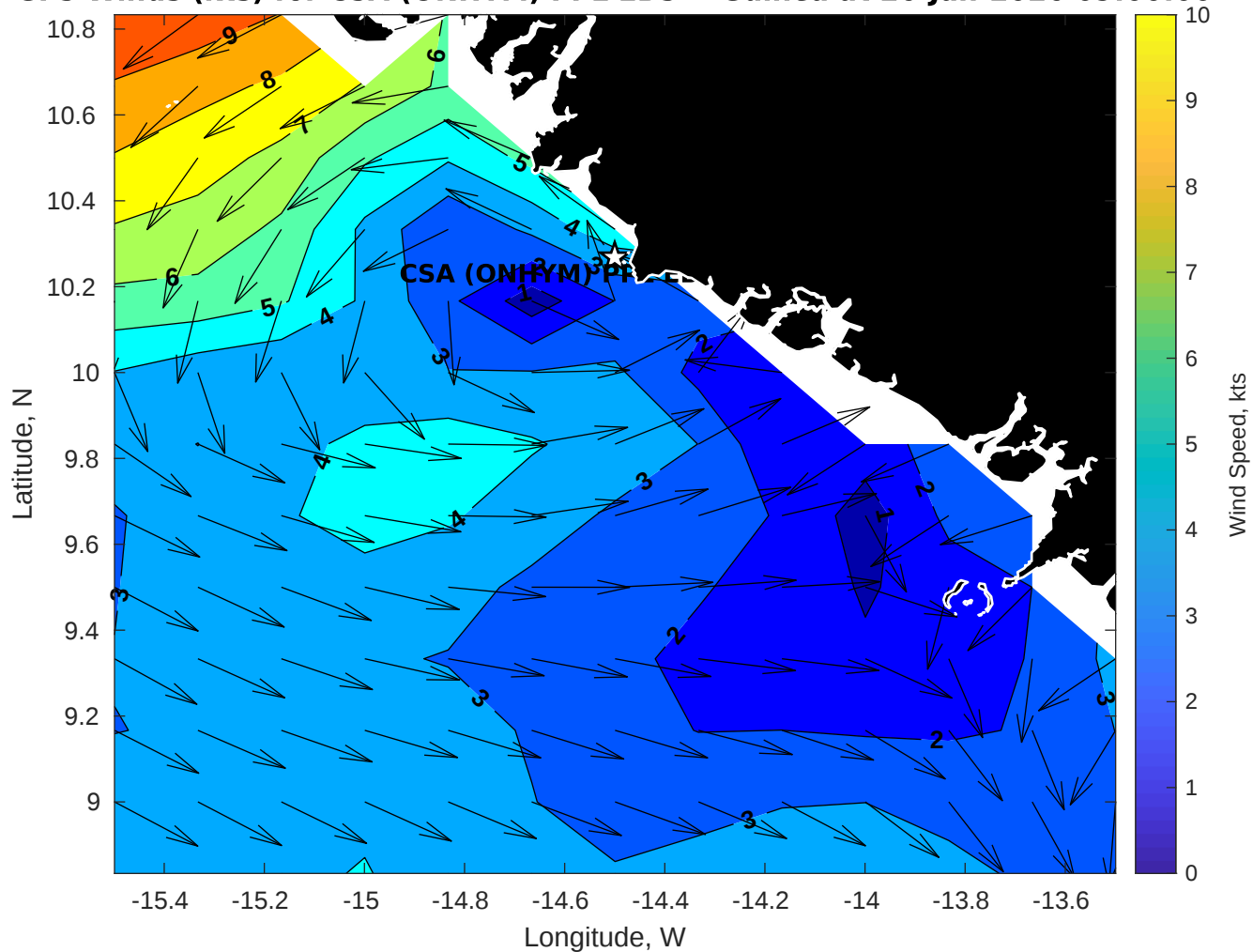
GFS Winds (kts) for CSA (ONHYM) PPL EBS - Guinea at 26-Jan-2026 09:00:00
