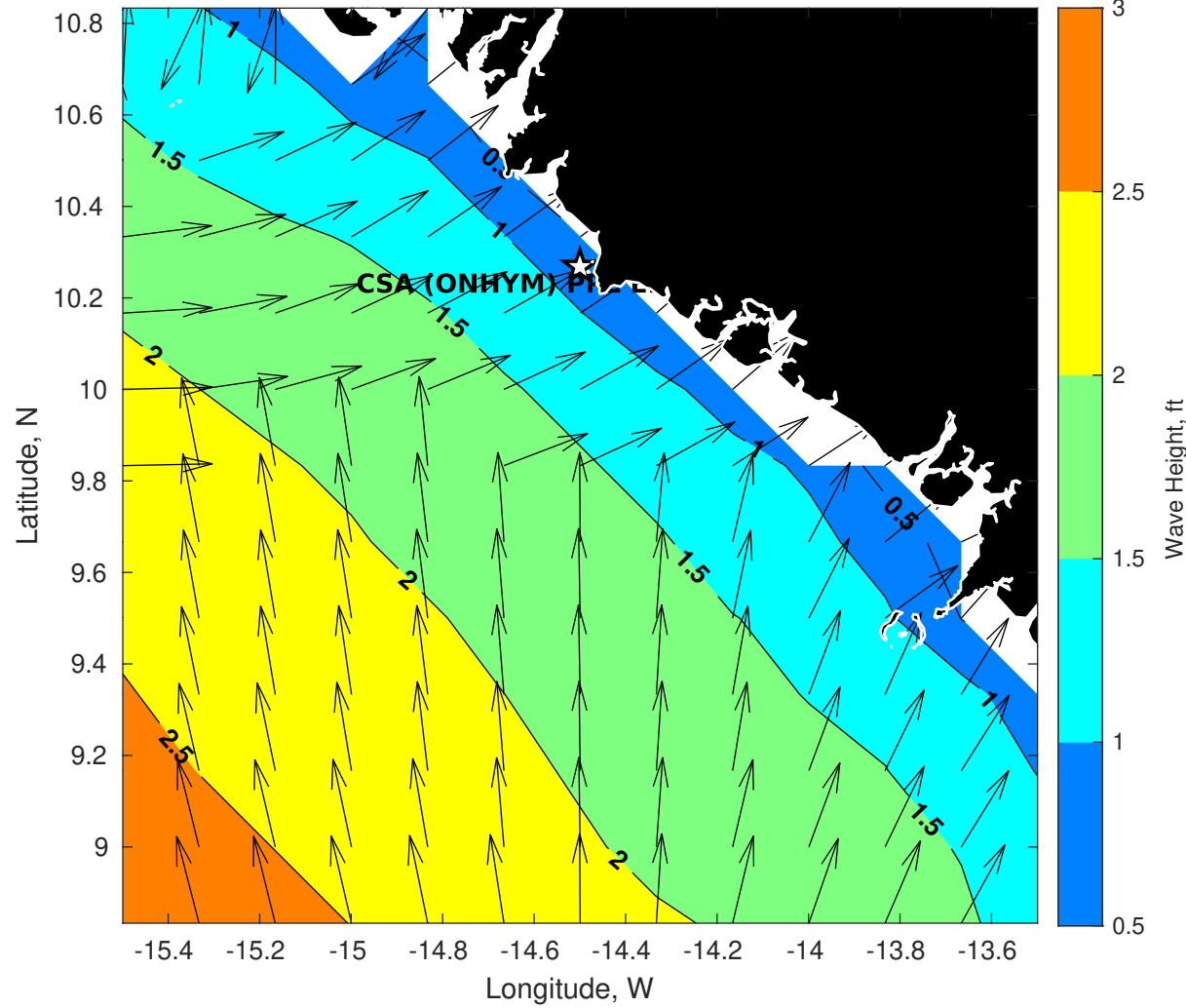
GFS Wave Height (ft) for CSA (ONHYM) PPL EBS - Guinea at 26-Jan-2026 09:00:00
