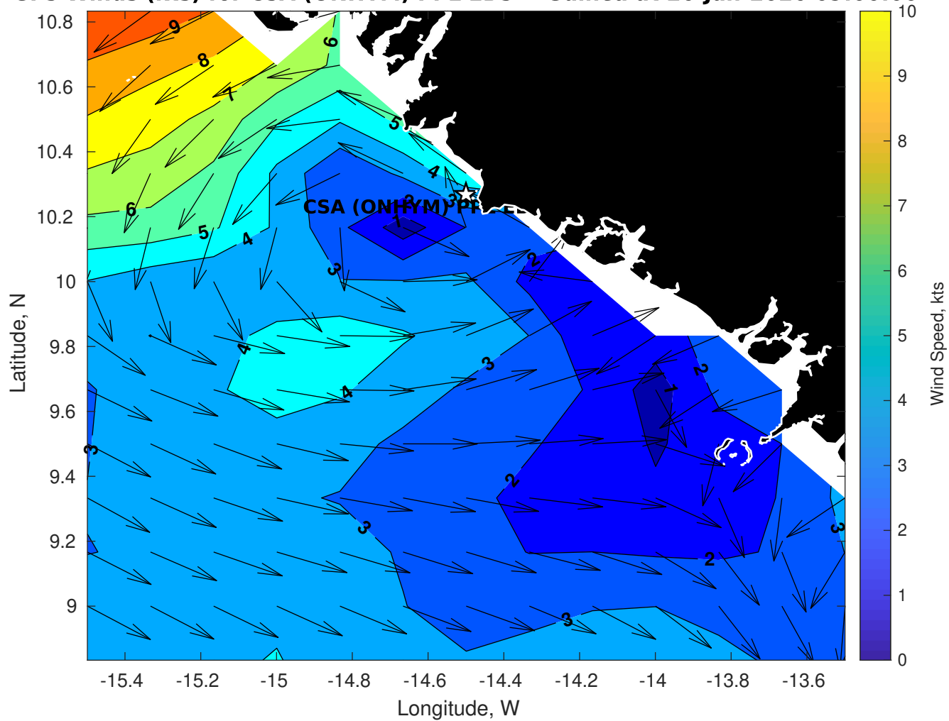
GFS Winds (kts) for CSA (ONHYM) PPL EBS - Guinea at 26-Jan-2026 09:00:00
