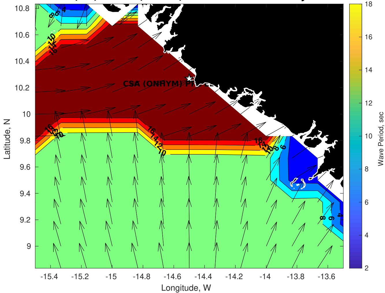
GFS Wave Period (sec) for CSA (ONHYM) PPL EBS - Guinea at 26-Jan-2026 09:00:00
