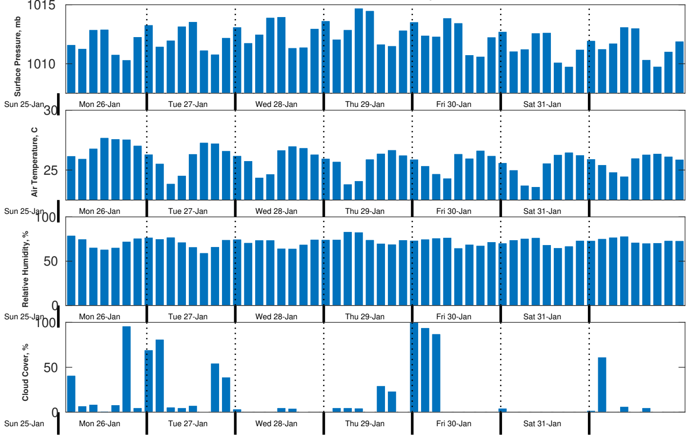
Met Forecast for CSA (ONHYM) PPL EBS - Guinea from 26-Jan-2026 00:00:00 to 02-Feb-2026 00:00:00
