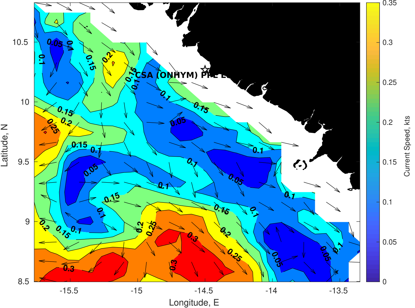
Surface Currents for CSA (ONHYM) PPL EBS - Guinea at 25-Jan-2026 00:00:00
