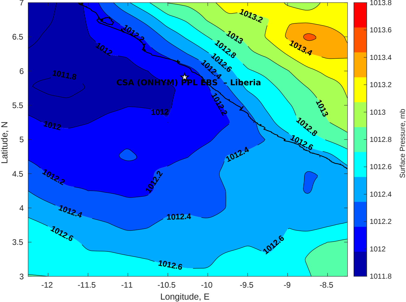
Surface Pressure (mb) for CSA (ONHYM) PPL EBS - Liberia at 26-Jan-2026 00:00:00
