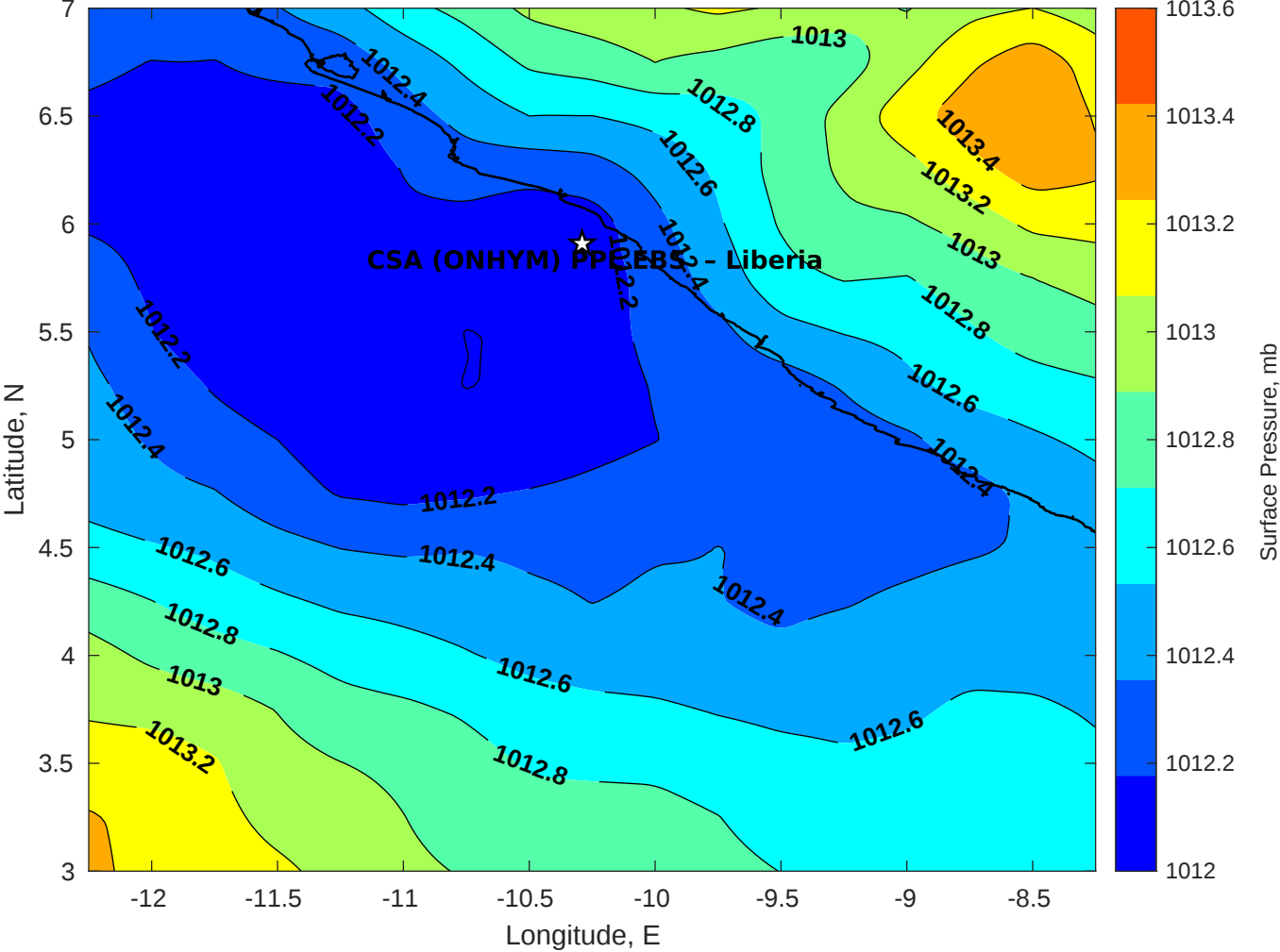
Surface Pressure (mb) for CSA (ONHYM) PPL EBS - Liberia at 27-Jan-2026 00:00:00
