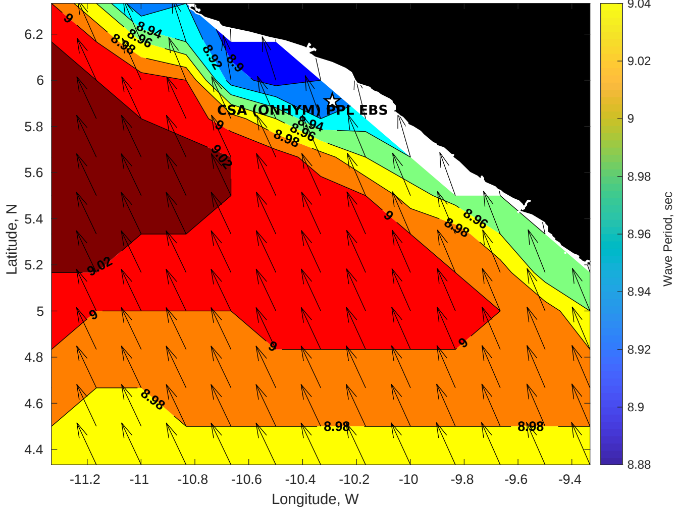
GFS Wave Period (sec) for CSA (ONHYM) PPL EBS - Liberia at 26-Jan-2026 09:00:00
