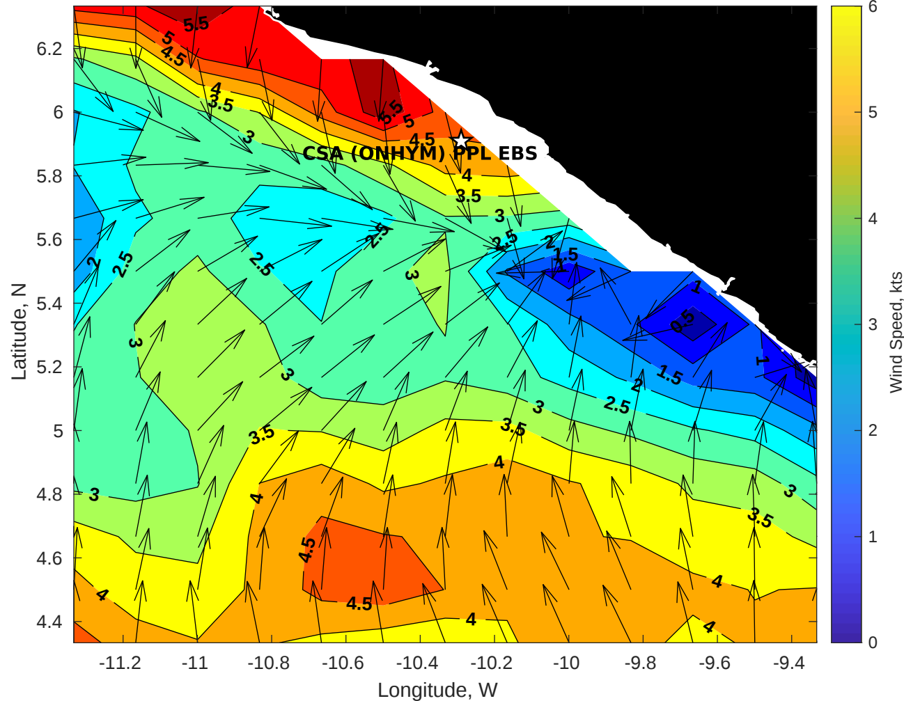
GFS Winds (kts) for CSA (ONHYM) PPL EBS - Liberia at 26-Jan-2026 09:00:00
