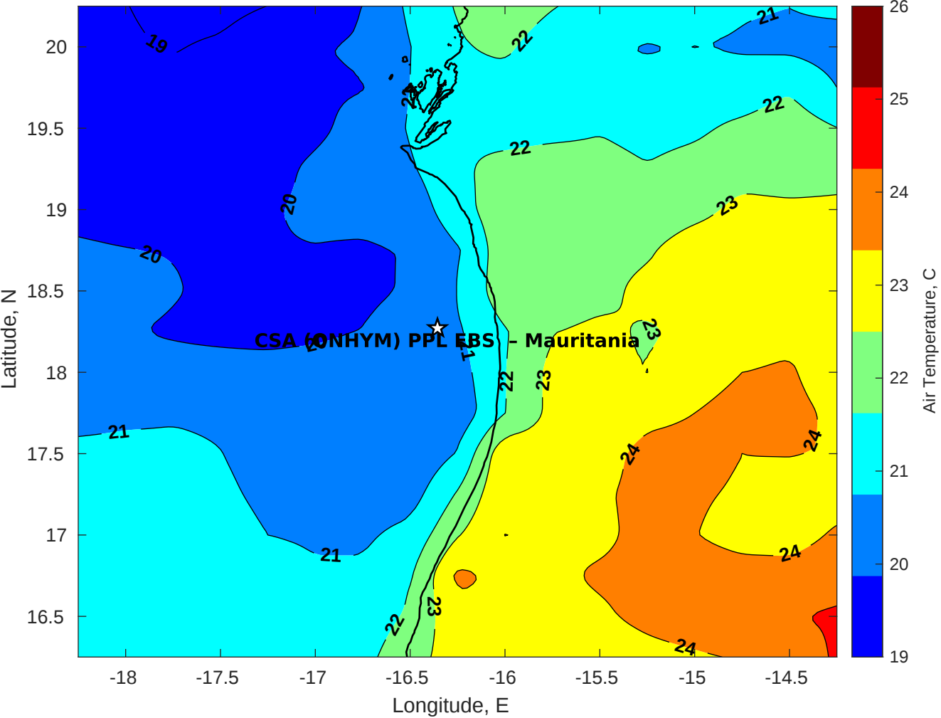
Air Temperature (C) for CSA (ONHYM) PPL EBS - Mauritania at 26-Jan-2026
