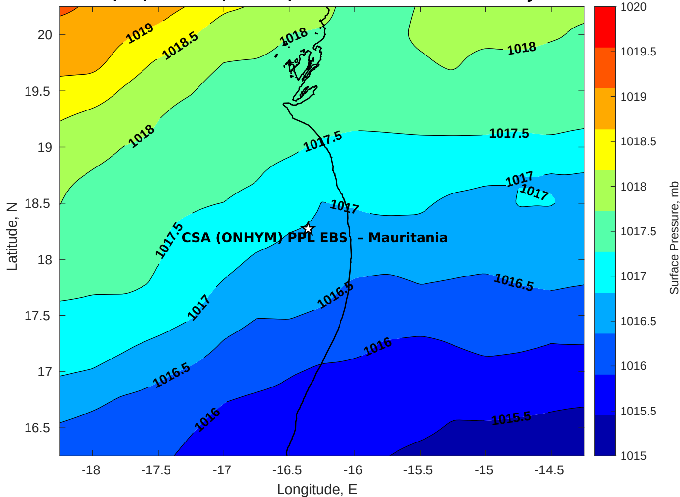
Surface Pressure (mb) for CSA (ONHYM) PPL EBS - Mauritania at 28-Jan-2026 00:00:00
