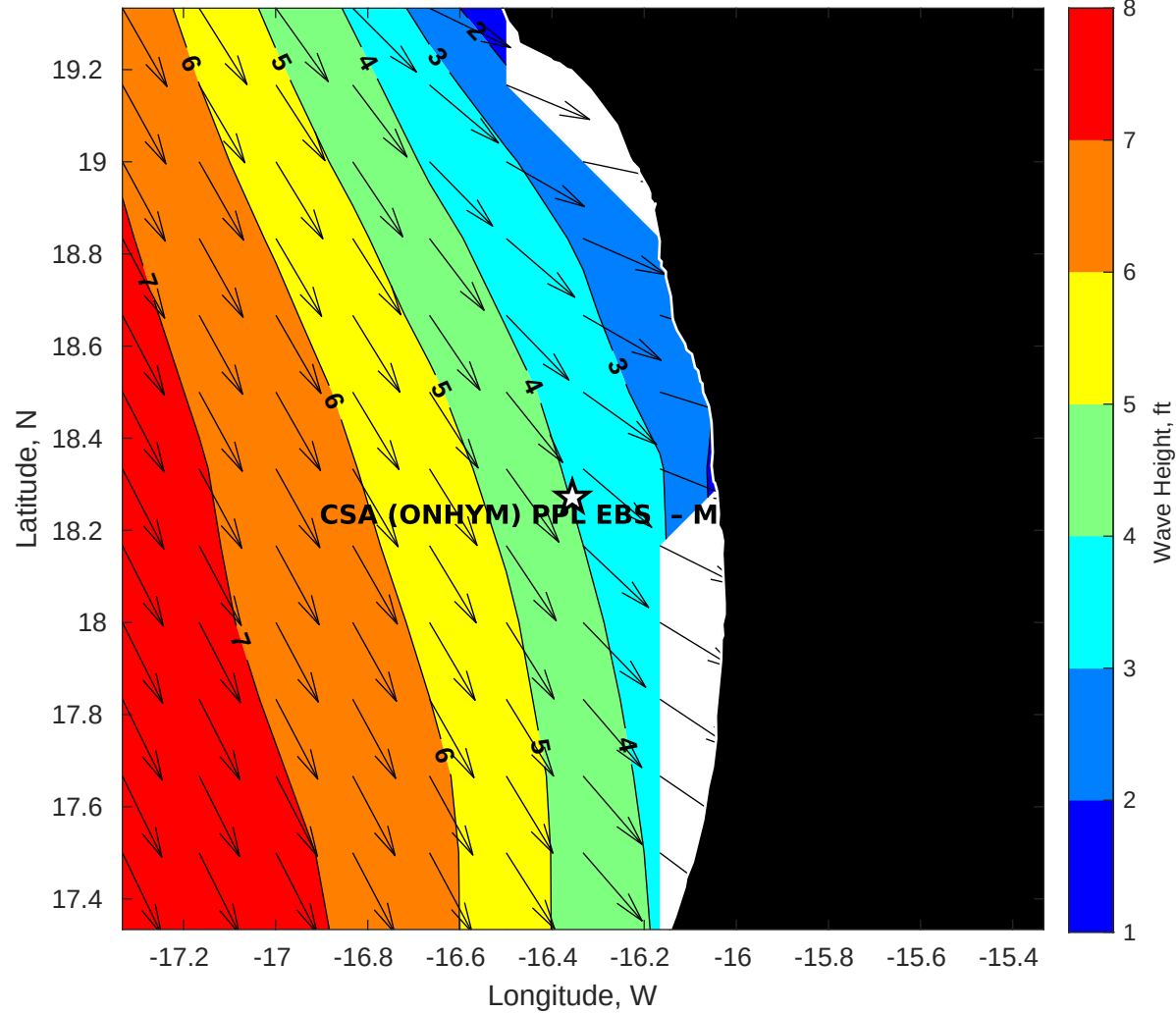
GFS Wave Height (ft) for CSA (ONHYM) PPL EBS - Mauritania at 26-Jan-2026 09:00:00
