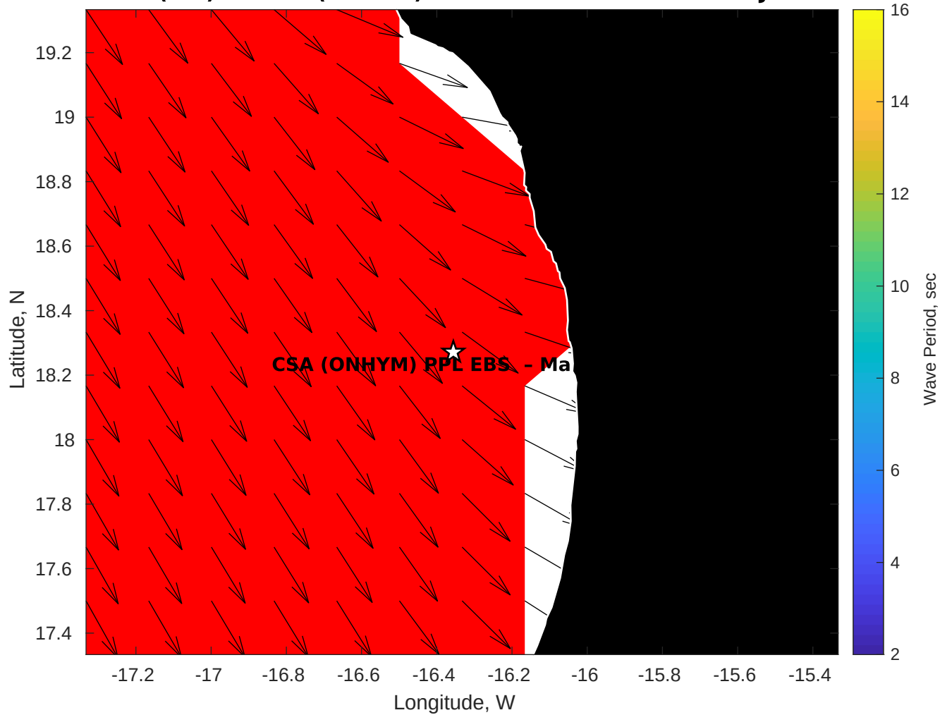
GFS Wave Period (sec) for CSA (ONHYM) PPL EBS - Mauritania at 26-Jan-2026 09:00:00
