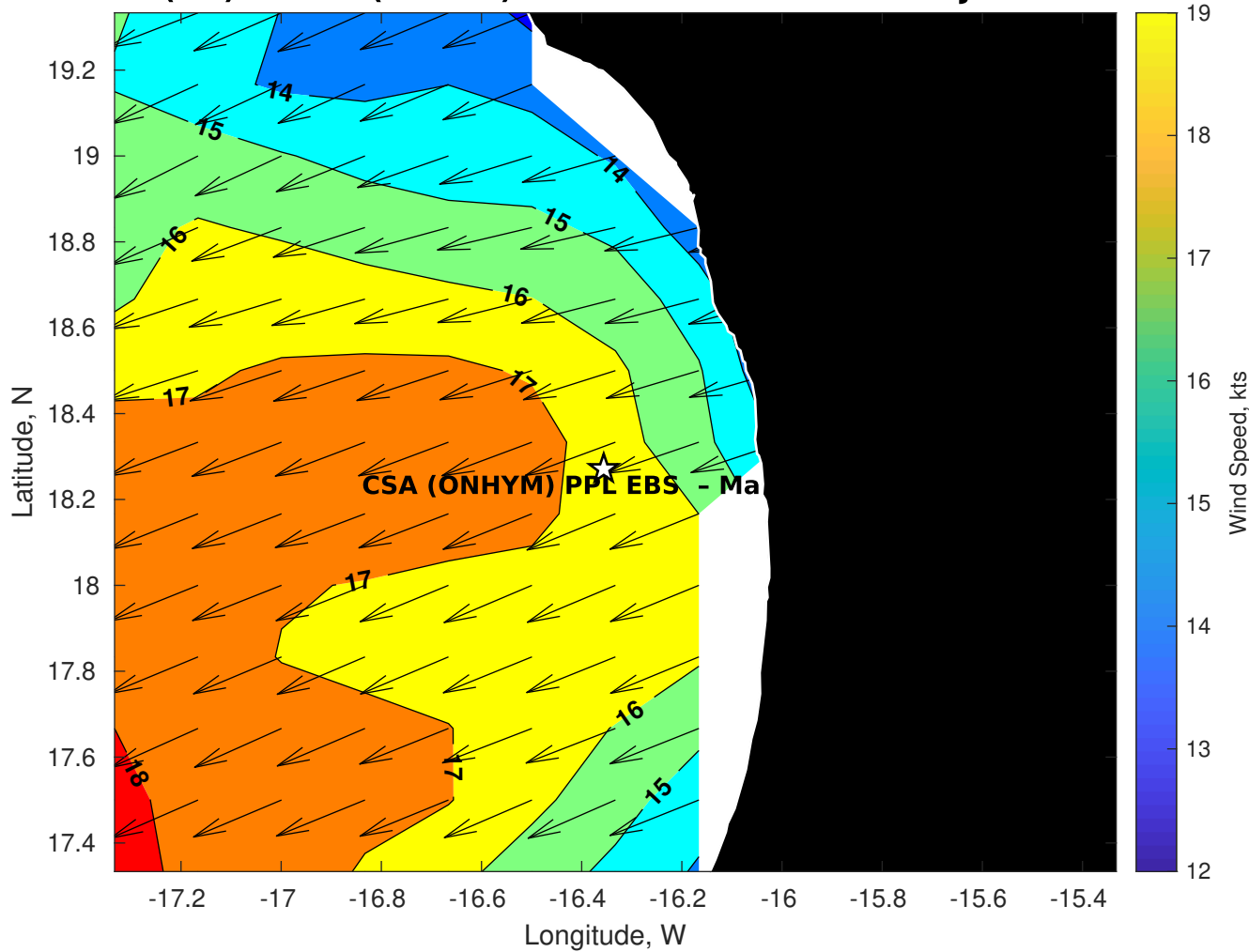
GFS Winds (kts) for CSA (ONHYM) PPL EBS - Mauritania at 26-Jan-2026 09:00:00
