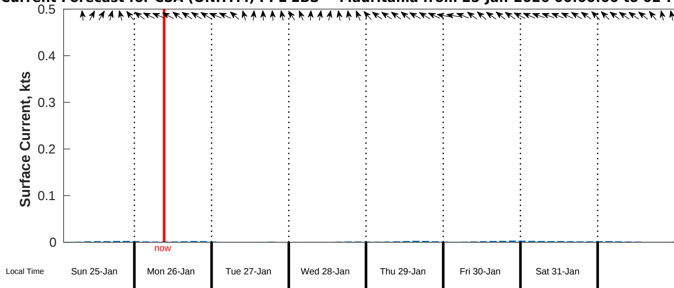
Surface Current Forecast for CSA (ONHYM) PPL EBS - Mauritania from 25-Jan-2026 00:00:00 to 02-Feb-2026 00:00:00
