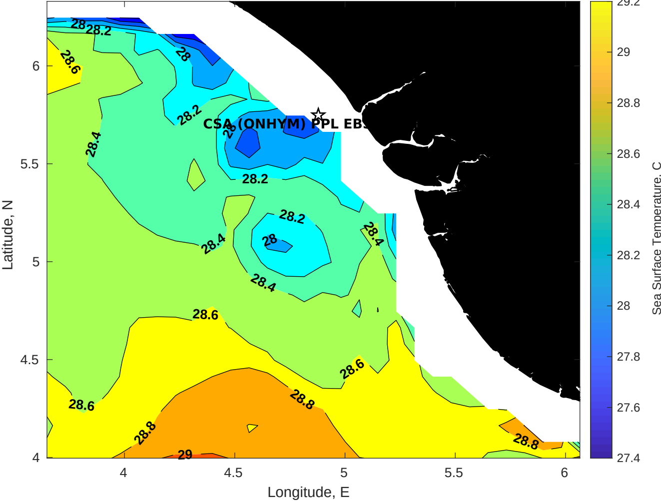
SST for CSA (ONHYM) PPL EBS - Nigeria at 25-Jan-2026 00:00:00
