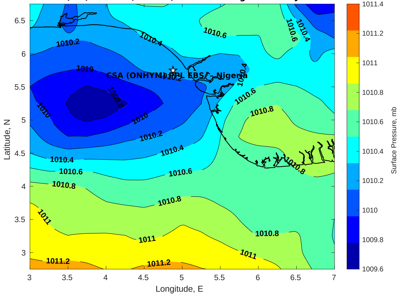
Surface Pressure (mb) for CSA (ONHYM) PPL EBS - Nigeria at 27-Jan-2026 00:00:00
