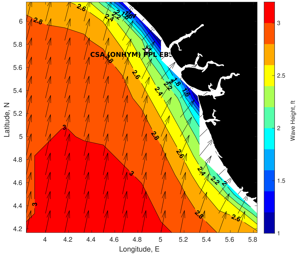
GFS Wave Height (ft) for CSA (ONHYM) PPL EBS - Nigeria at 26-Jan-2026 09:00:00
