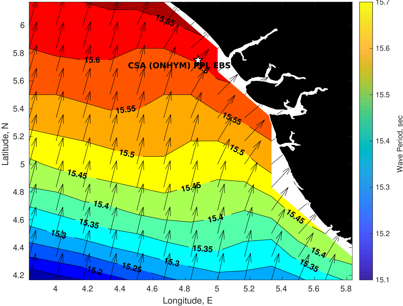
GFS Wave Period (sec) for CSA (ONHYM) PPL EBS - Nigeria at 26-Jan-2026 09:00:00
