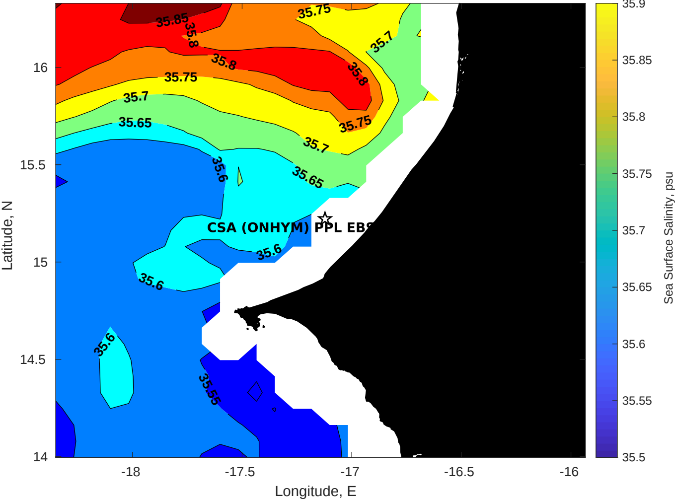
Surface Salinity for CSA (ONHYM) PPL EBS - Senegal at 25-Jan-2026 00:00:00
