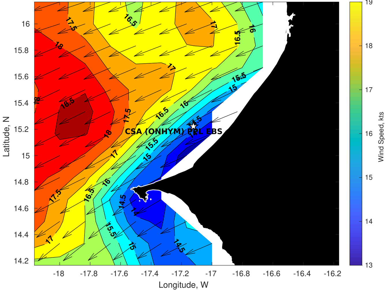
GFS Winds (kts) for CSA (ONHYM) PPL EBS - Senegal at 26-Jan-2026 09:00:00
