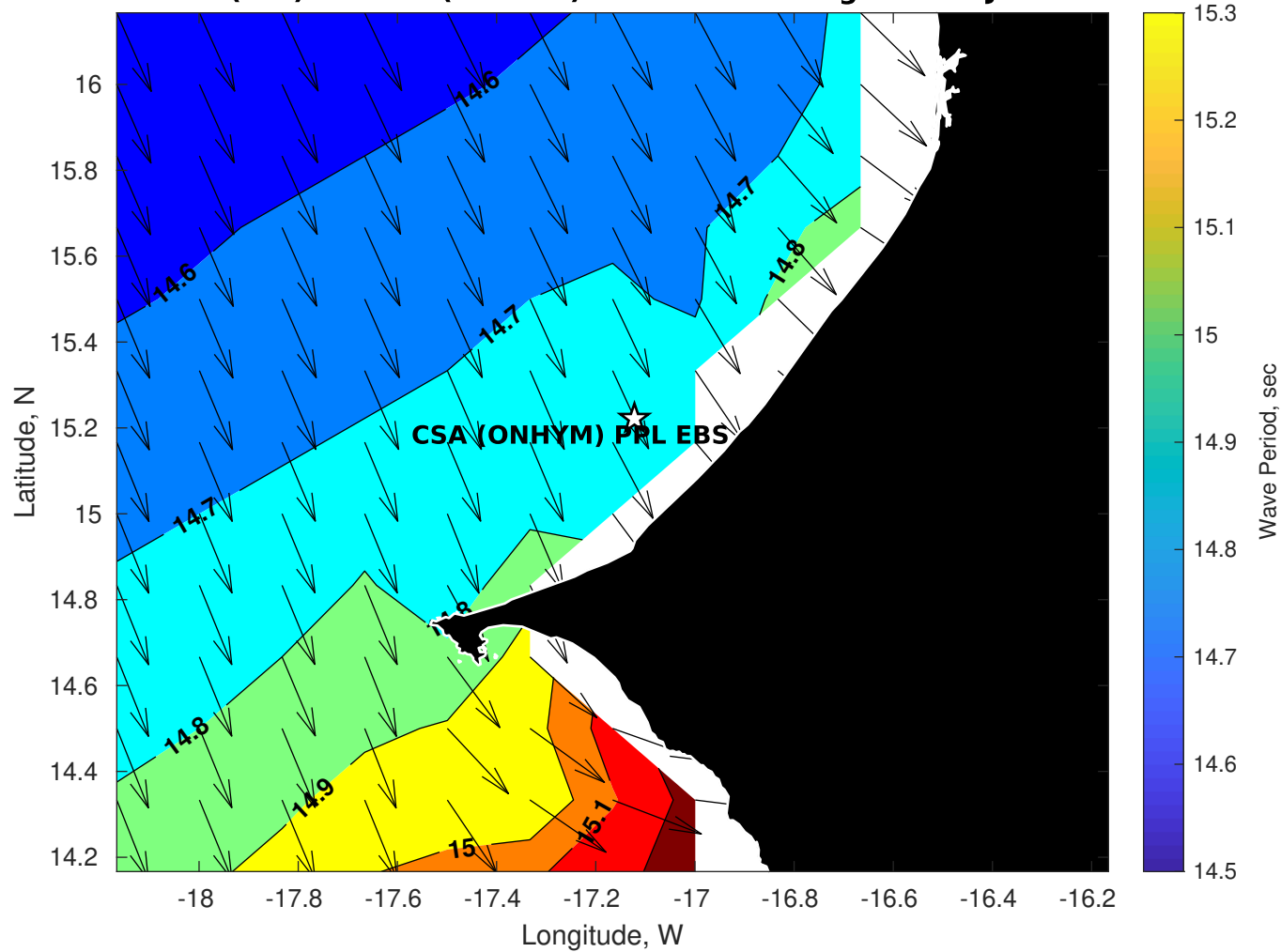
GFS Wave Period (sec) for CSA (ONHYM) PPL EBS - Senegal at 26-Jan-2026 09:00:00
