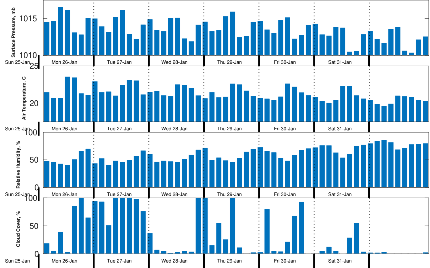
Met Forecast for CSA (ONHYM) PPL EBS - Senegal from 26-Jan-2026 00:00:00 to 02-Feb-2026 00:00:00
