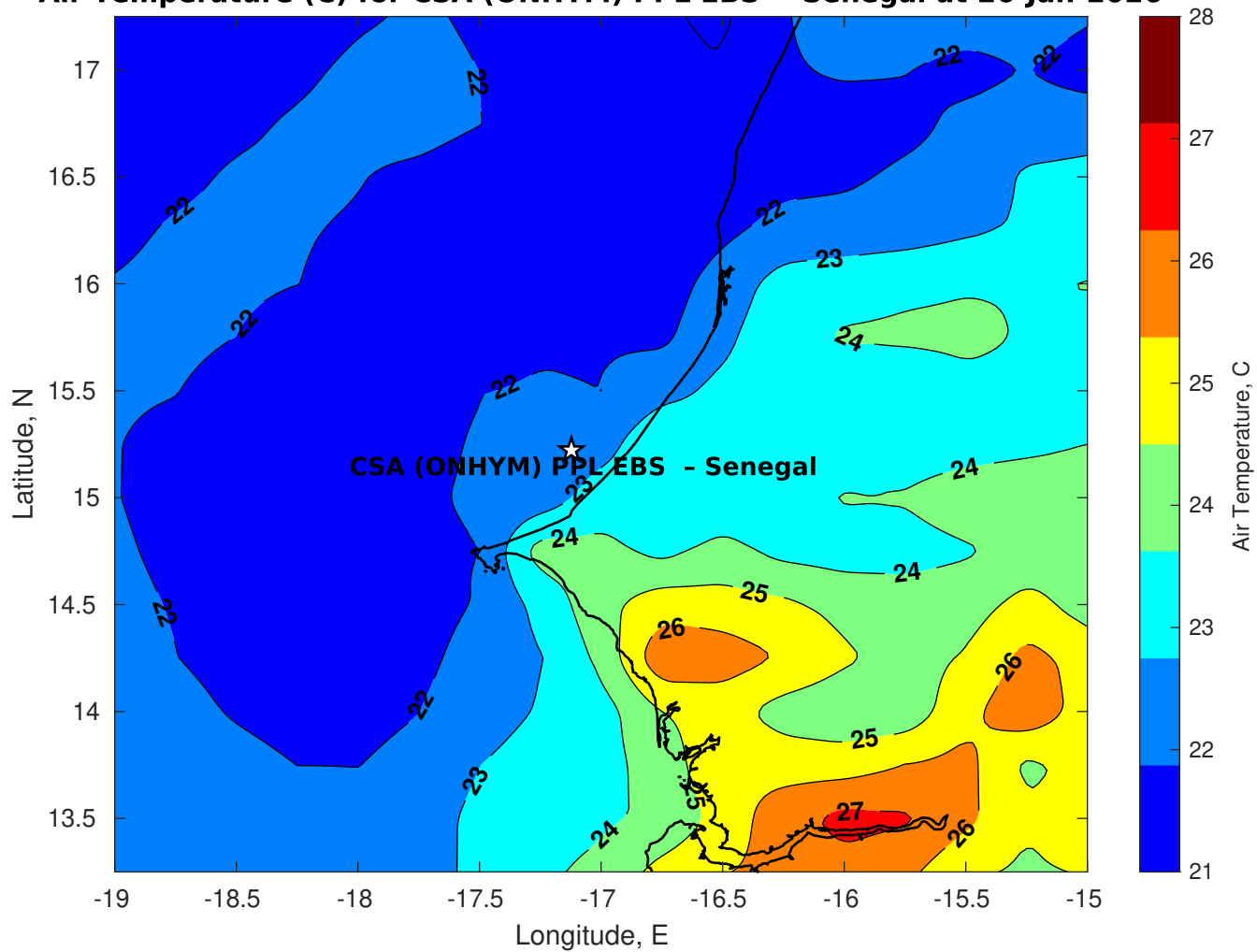
Air Temperature (C) for CSA (ONHYM) PPL EBS - Senegal at 26-Jan-2026
