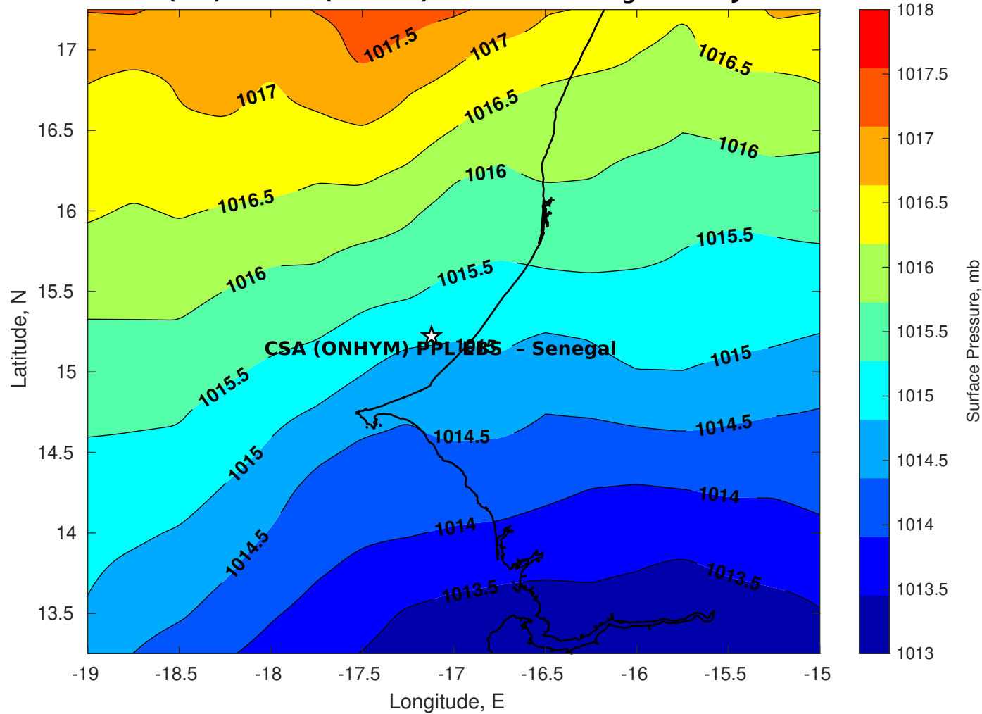
Surface Pressure (mb) for CSA (ONHYM) PPL EBS - Senegal at 27-Jan-2026 00:00:00
