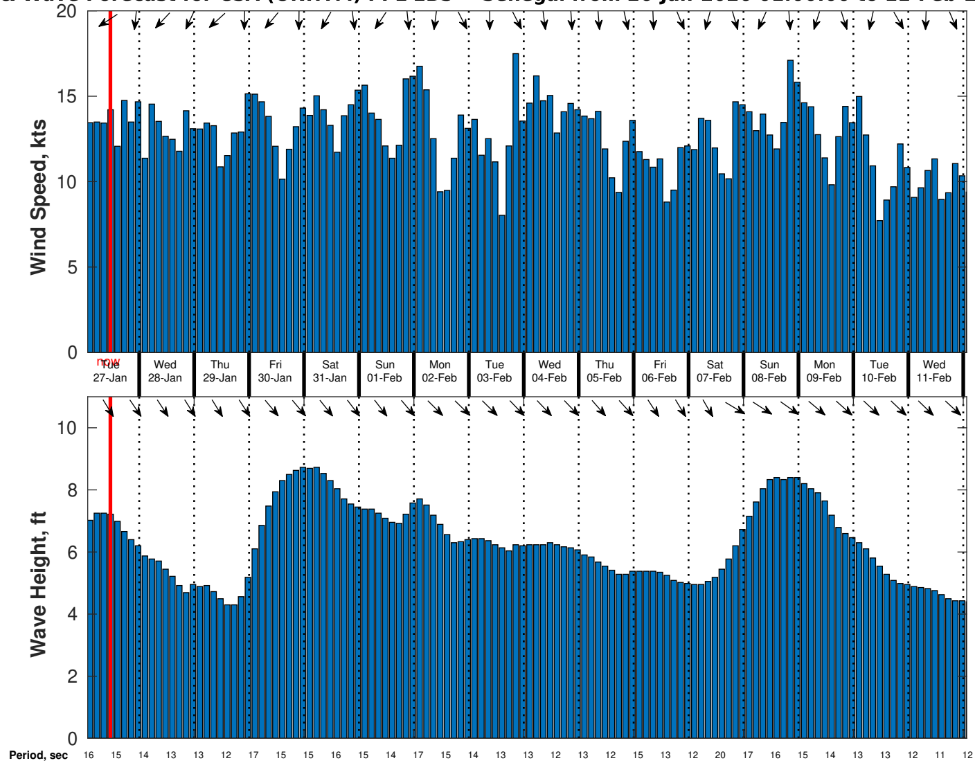
Wind & Wave Forecast for CSA (ONHYM) PPL EBS - Senegal from 26-Jan-2026 01:00:00 to 11-Feb-2026 01:00:00
