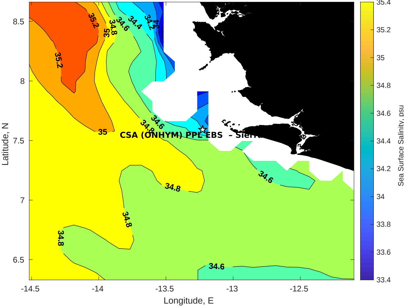
Surface Salinity for CSA (ONHYM) PPL EBS - Sierra Leone at 25-Jan-2026 00:00:00
