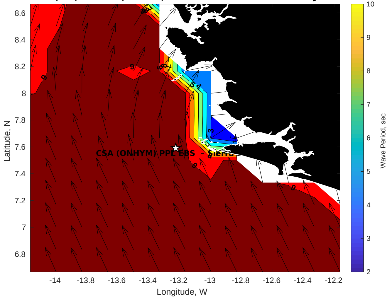
GFS Wave Period (sec) for CSA (ONHYM) PPL EBS - Sierra Leone at 26-Jan-2026 09:00:00
