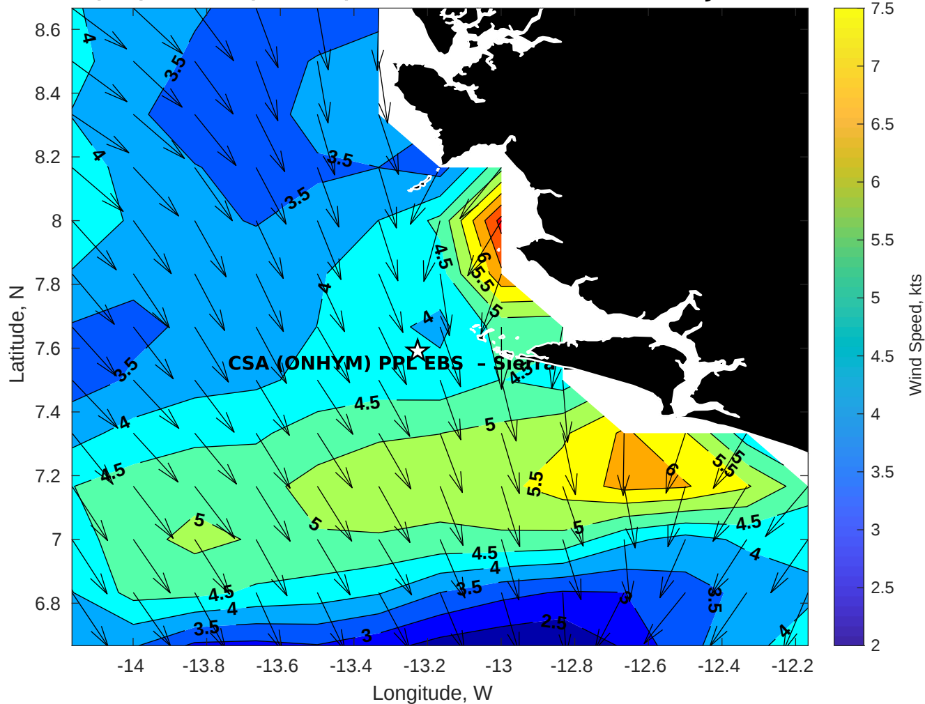
GFS Winds (kts) for CSA (ONHYM) PPL EBS - Sierra Leone at 26-Jan-2026 09:00:00
