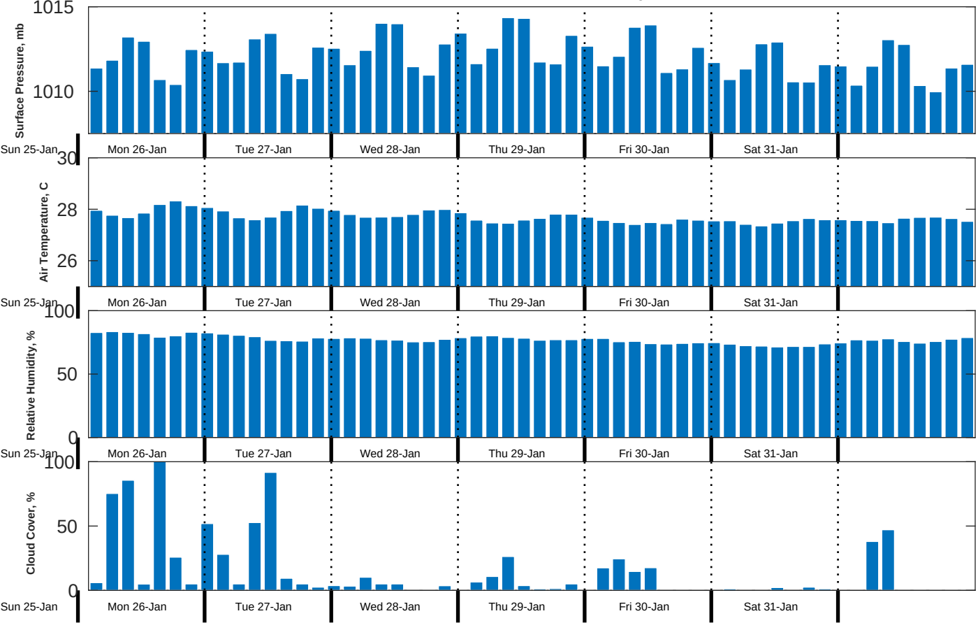
Met Forecast for CSA (ONHYM) PPL EBS - Sierra Leone from 26-Jan-2026 00:00:00 to 02-Feb-2026 00:00:00
