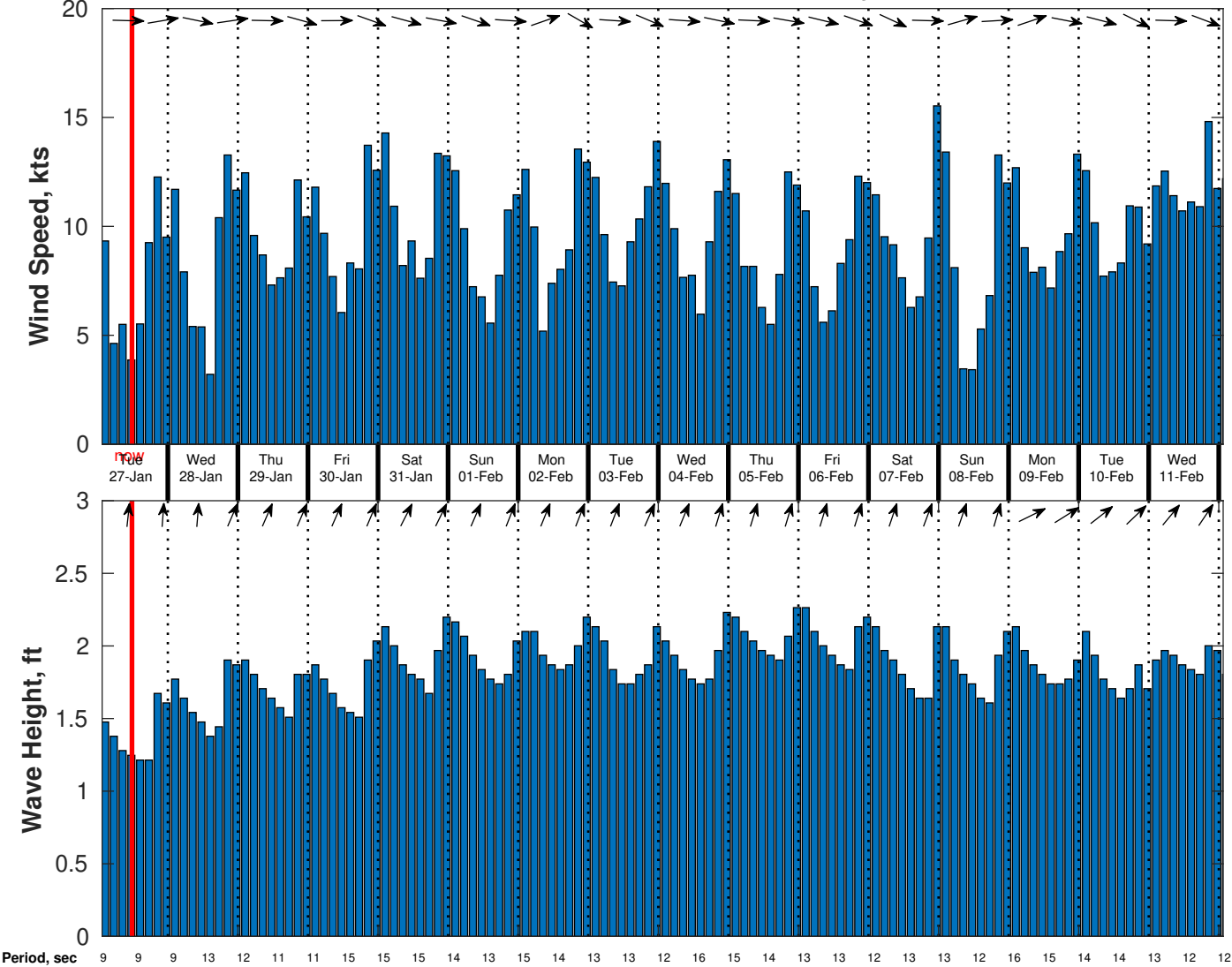
Wind & Wave Forecast for CSA (ONHYM) PPL EBS - Sierra Leone from 26-Jan-2026 01:00:00 to 11-Feb-2026 01:00:00
