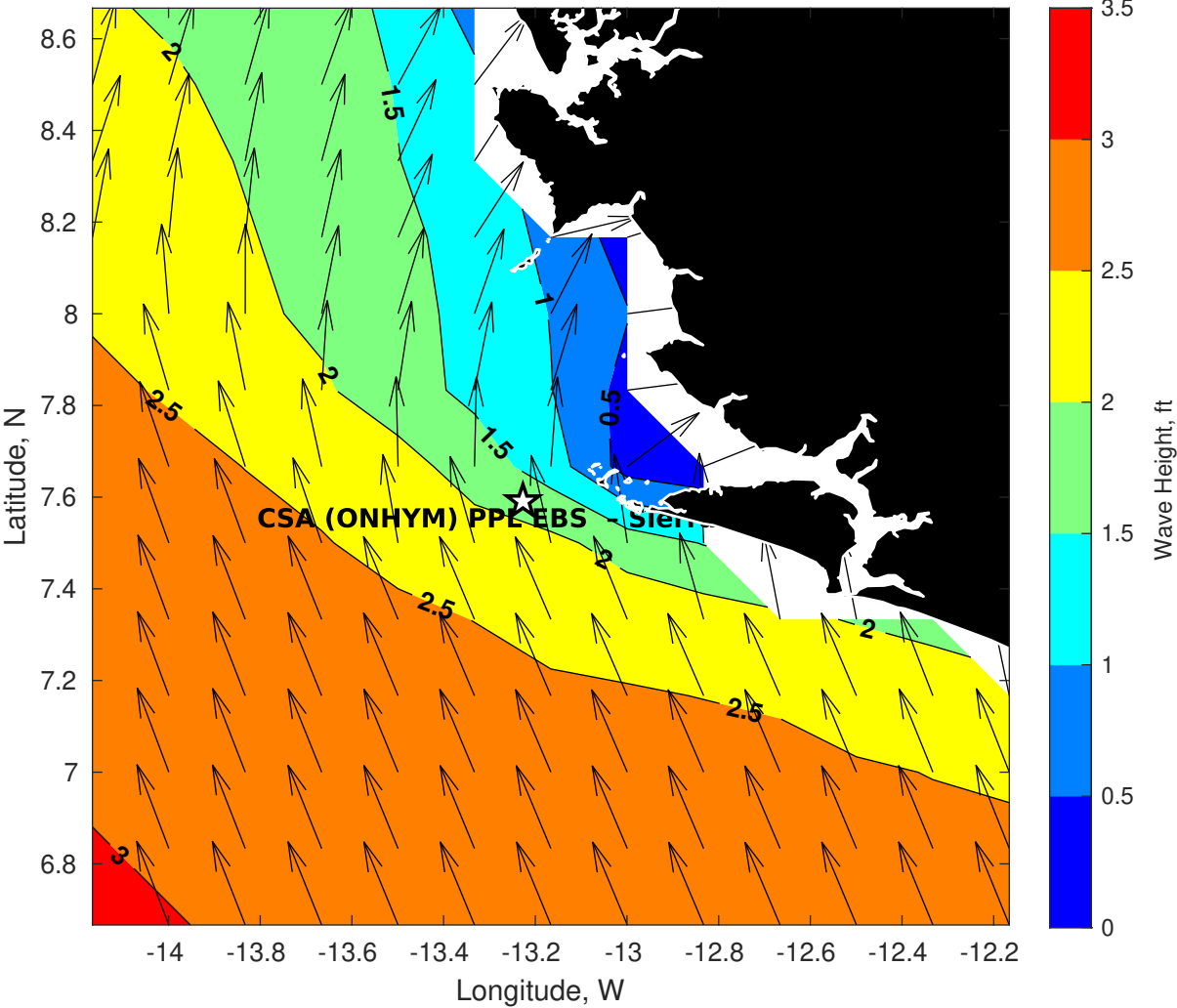
GFS Wave Height (ft) for CSA (ONHYM) PPL EBS - Sierra Leone at 26-Jan-2026 09:00:00
