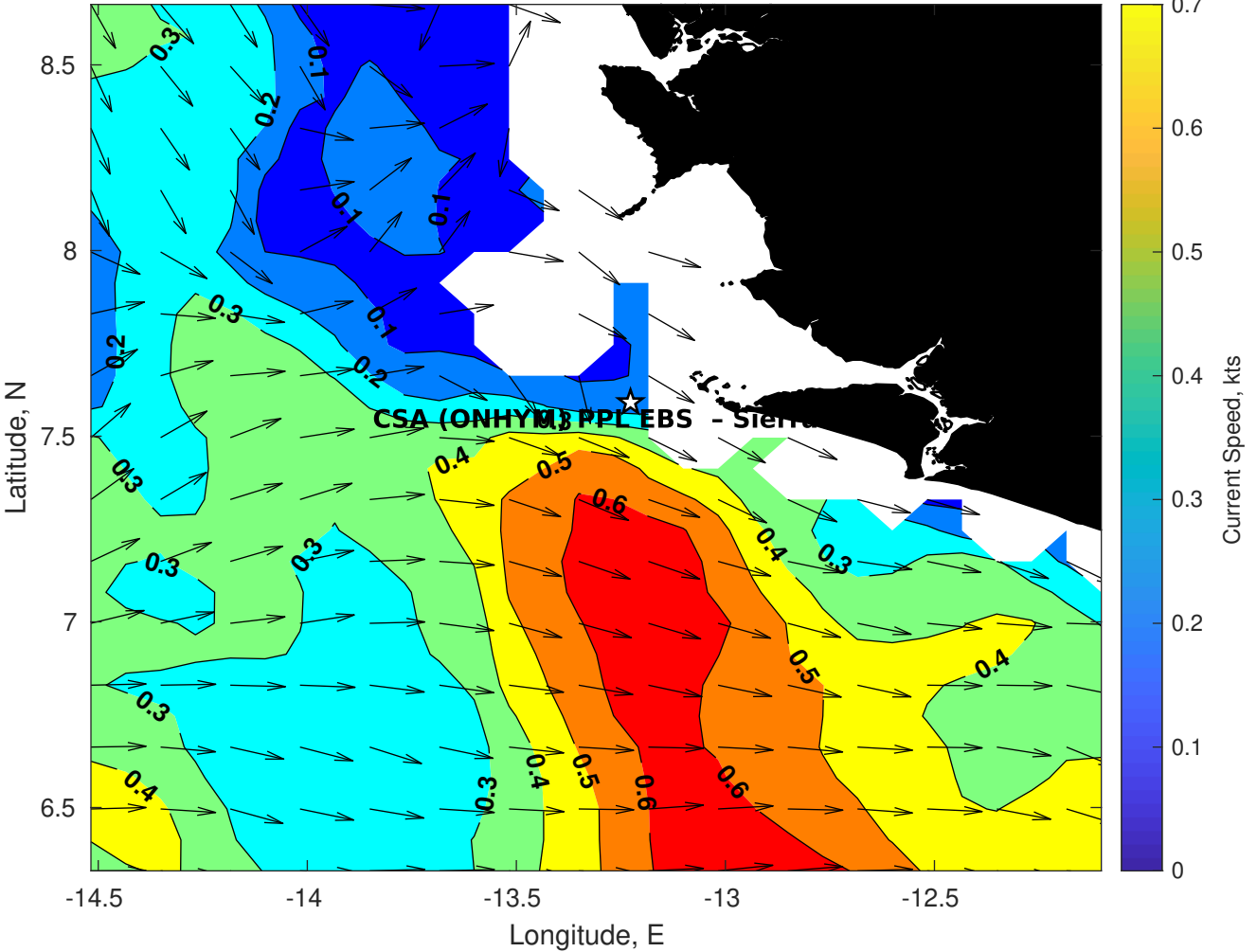
Surface Currents for CSA (ONHYM) PPL EBS - Sierra Leone at 25-Jan-2026 00:00:00
