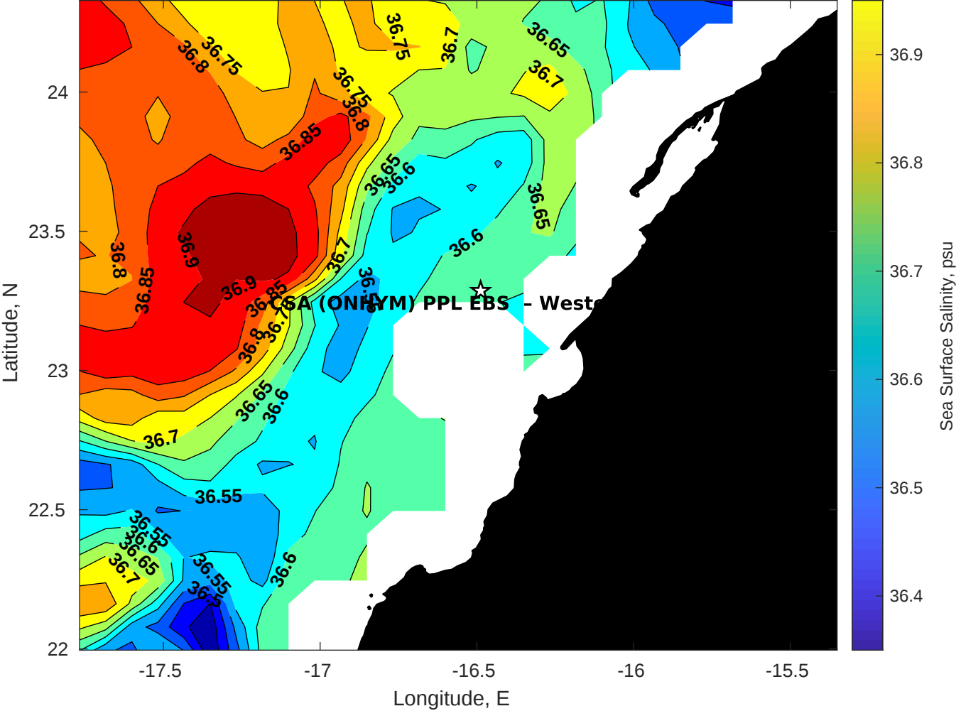
Surface Salinity for CSA (ONHYM) PPL EBS - Western Sahara at 25-Jan-2026 00:00:00
