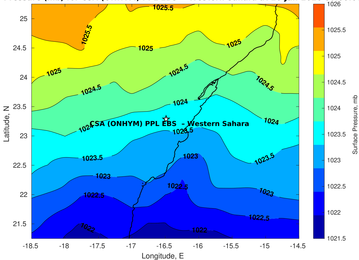
Surface Pressure (mb) for CSA (ONHYM) PPL EBS - Western Sahara at 26-Jan-2026 00:00:00
