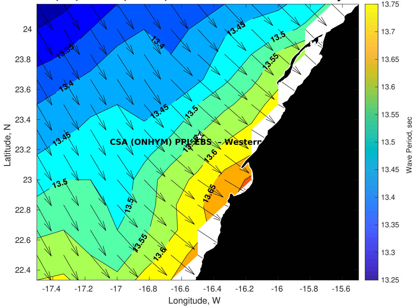
GFS Wave Period (sec) for CSA (ONHYM) PPL EBS - Western Sahara at 26-Jan-2026 09:00:00
