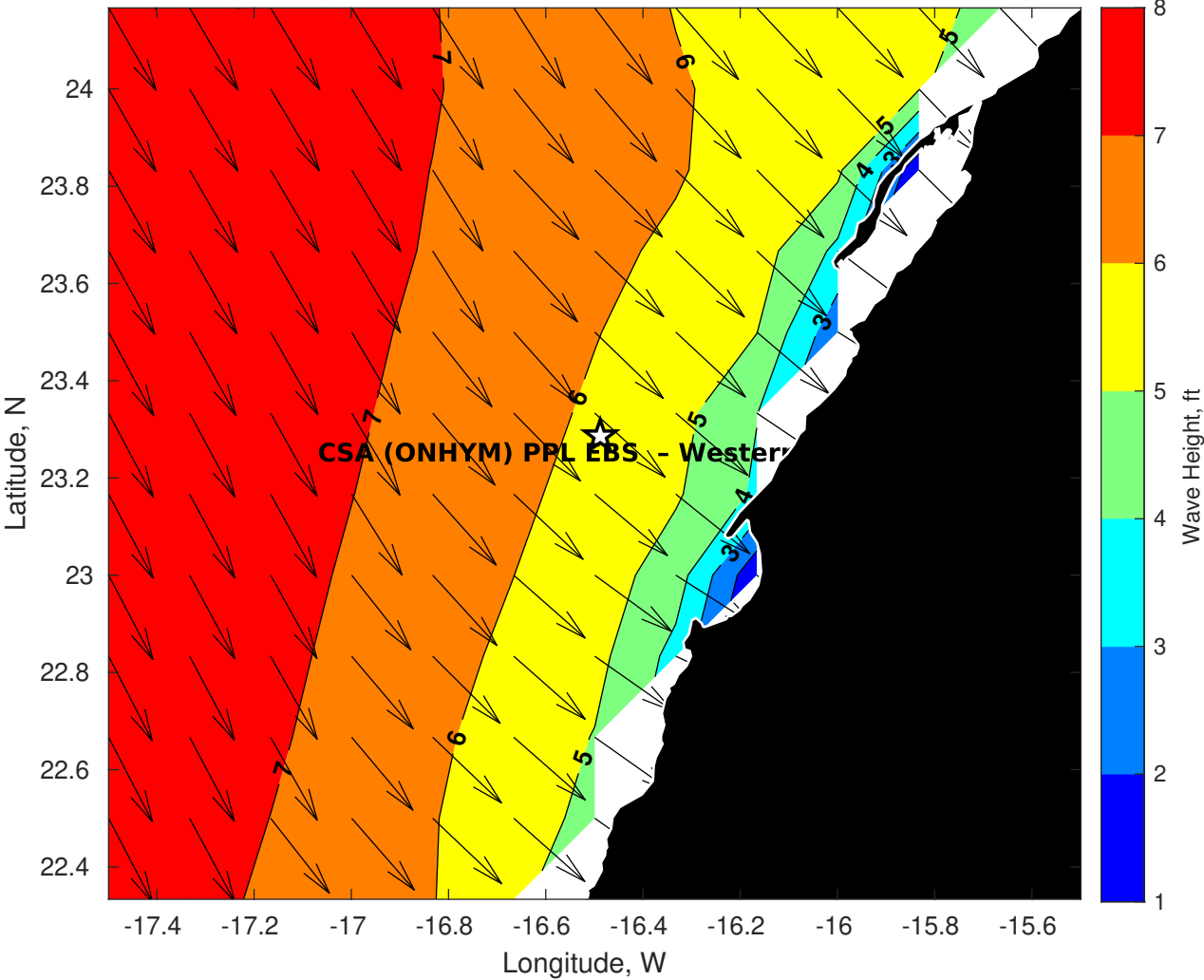
GFS Wave Height (ft) for CSA (ONHYM) PPL EBS - Western Sahara at 26-Jan-2026 09:00:00
