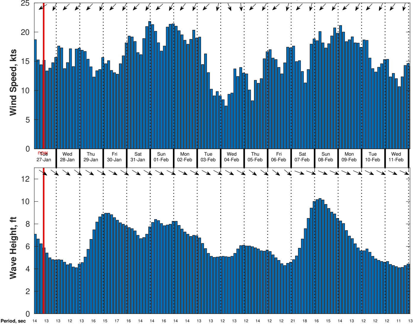
Wind & Wave Forecast for CSA (ONHYM) PPL EBS - Western Sahara from 26-Jan-2026 01:00:00 to 11-Feb-2026 01:00:00
