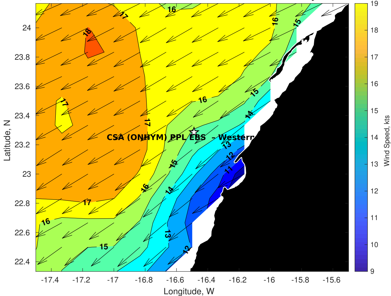
GFS Winds (kts) for CSA (ONHYM) PPL EBS - Western Sahara at 26-Jan-2026 09:00:00
