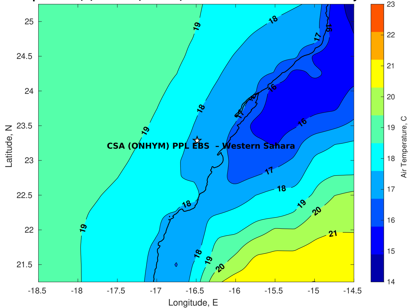
Air Temperature (C) for CSA (ONHYM) PPL EBS - Western Sahara at 26-Jan-2026
