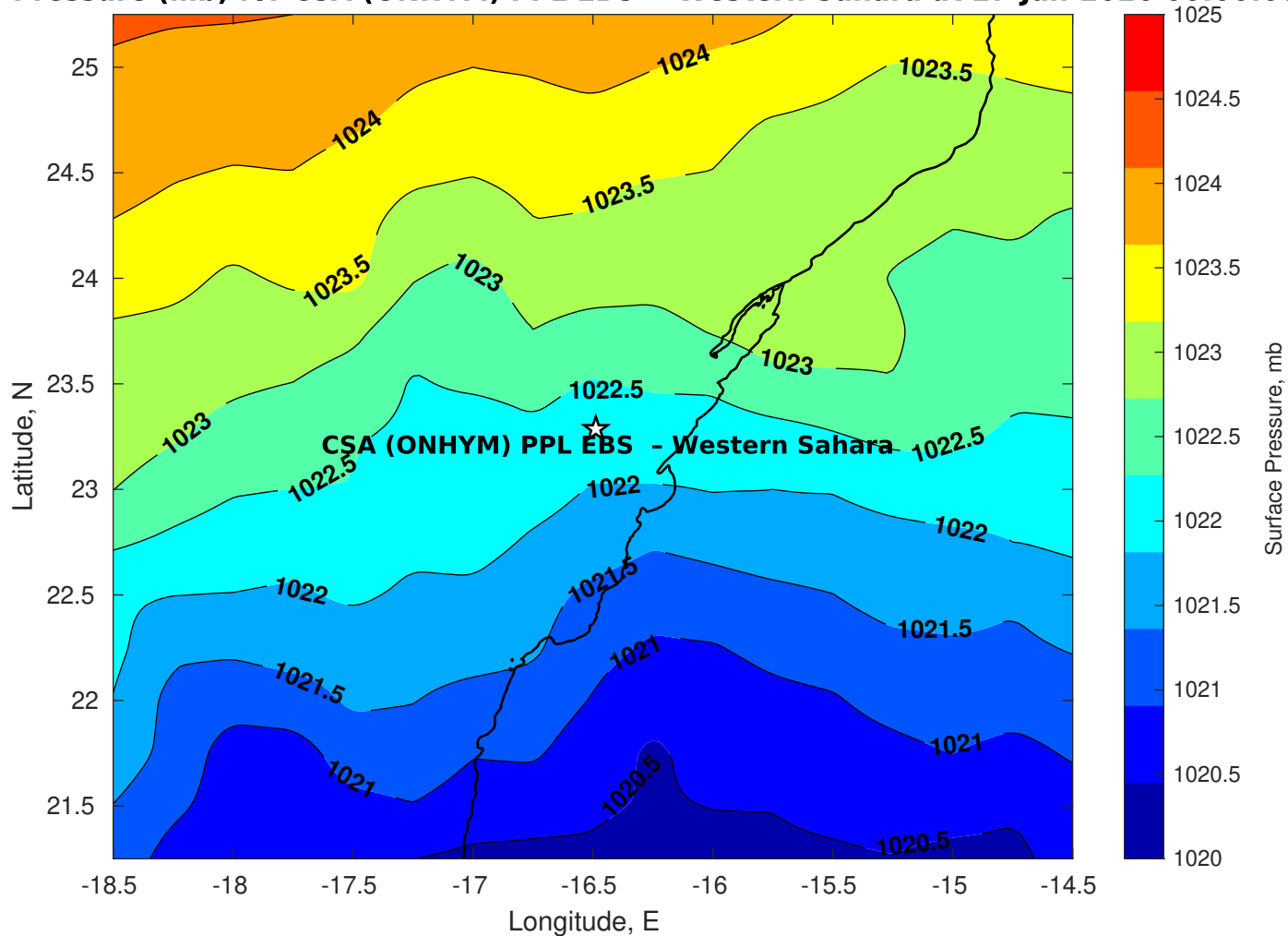
Surface Pressure (mb) for CSA (ONHYM) PPL EBS - Western Sahara at 27-Jan-2026 00:00:00
