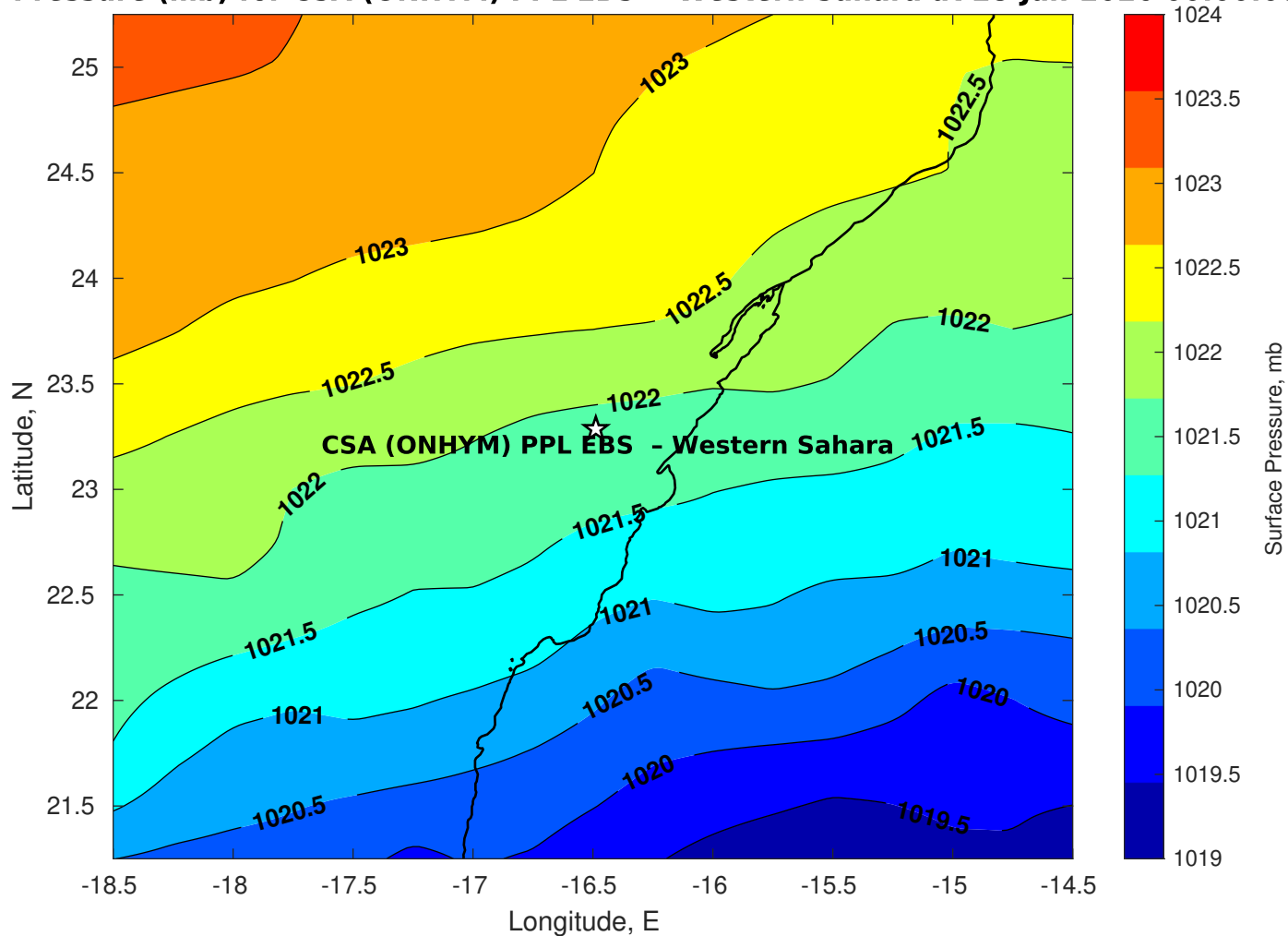
Surface Pressure (mb) for CSA (ONHYM) PPL EBS - Western Sahara at 28-Jan-2026 00:00:00
