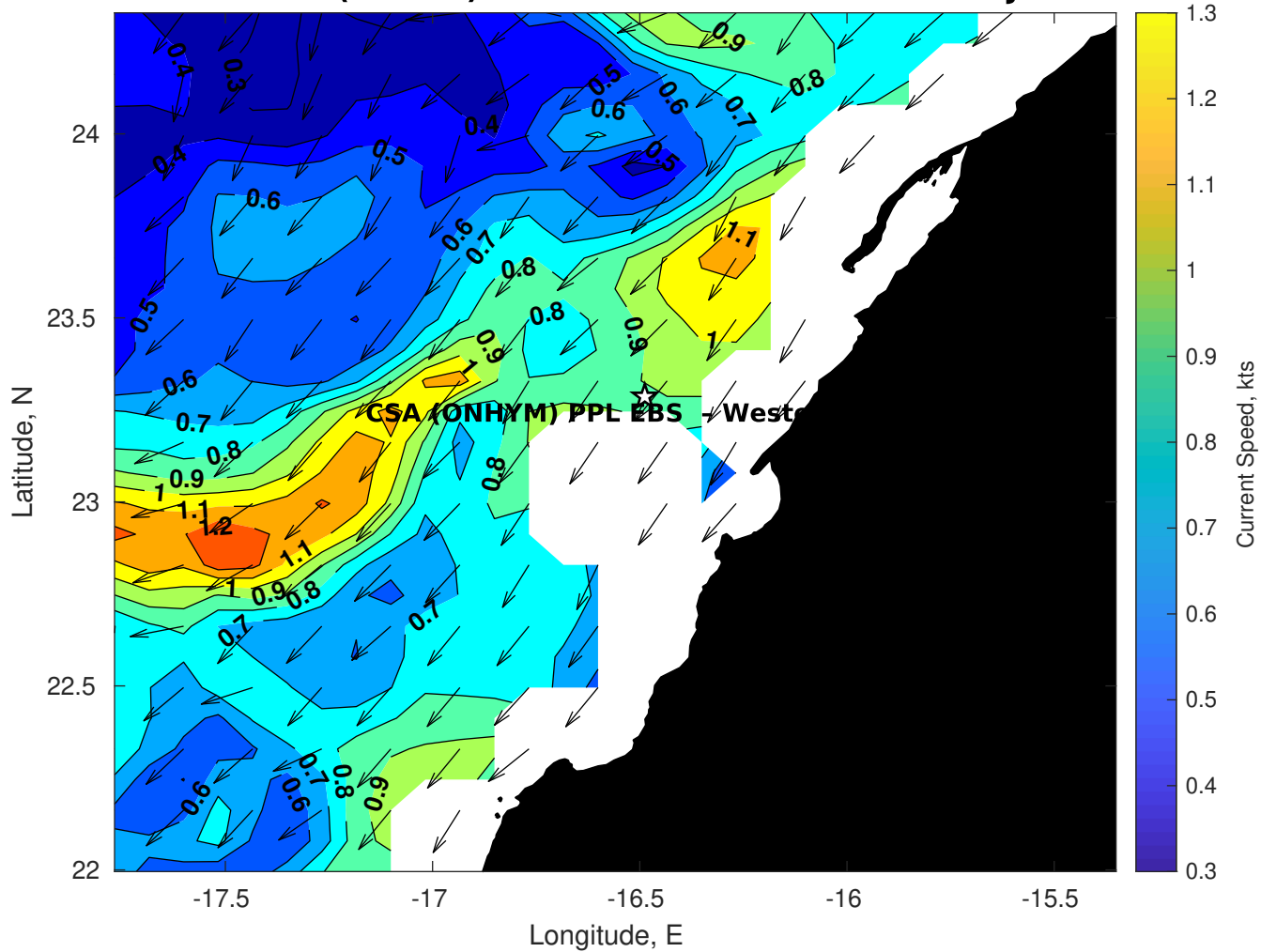
Surface Currents for CSA (ONHYM) PPL EBS - Western Sahara at 25-Jan-2026 00:00:00
