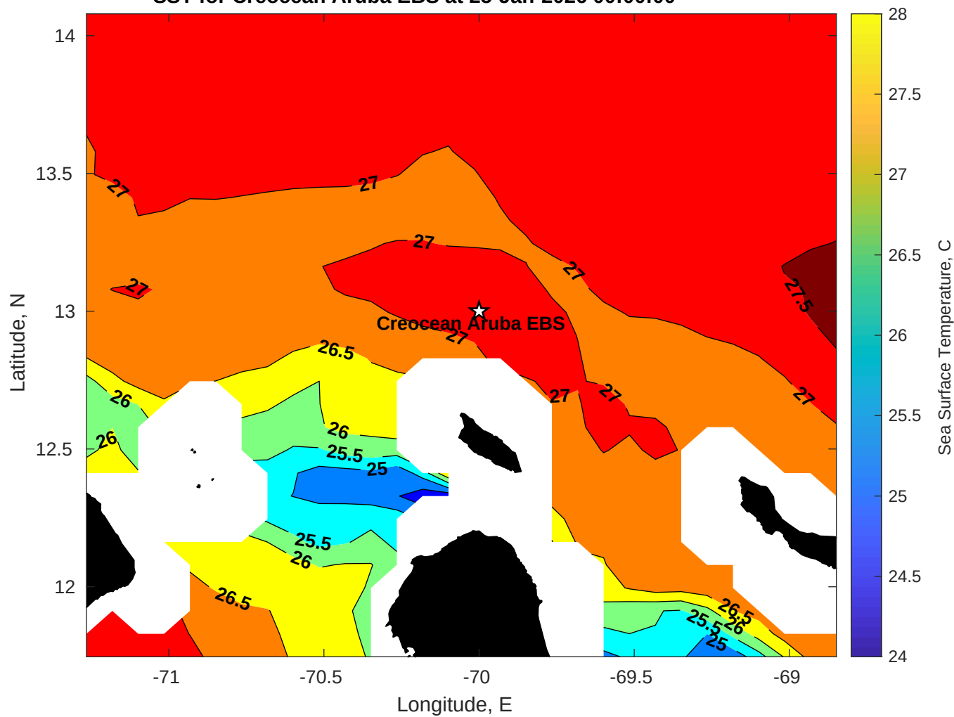
SST for Creoccean Aruba EBS at 25-Jan-2026 00:00:00
