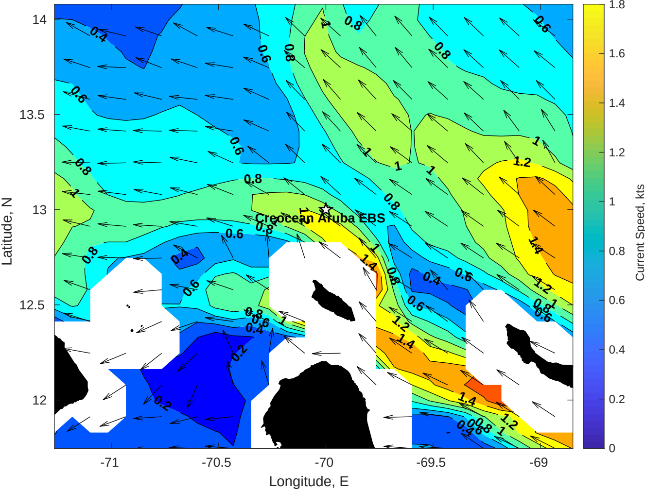
Surface Currents for Creoccean Aruba EBS at 25-Jan-2026 00:00:00
