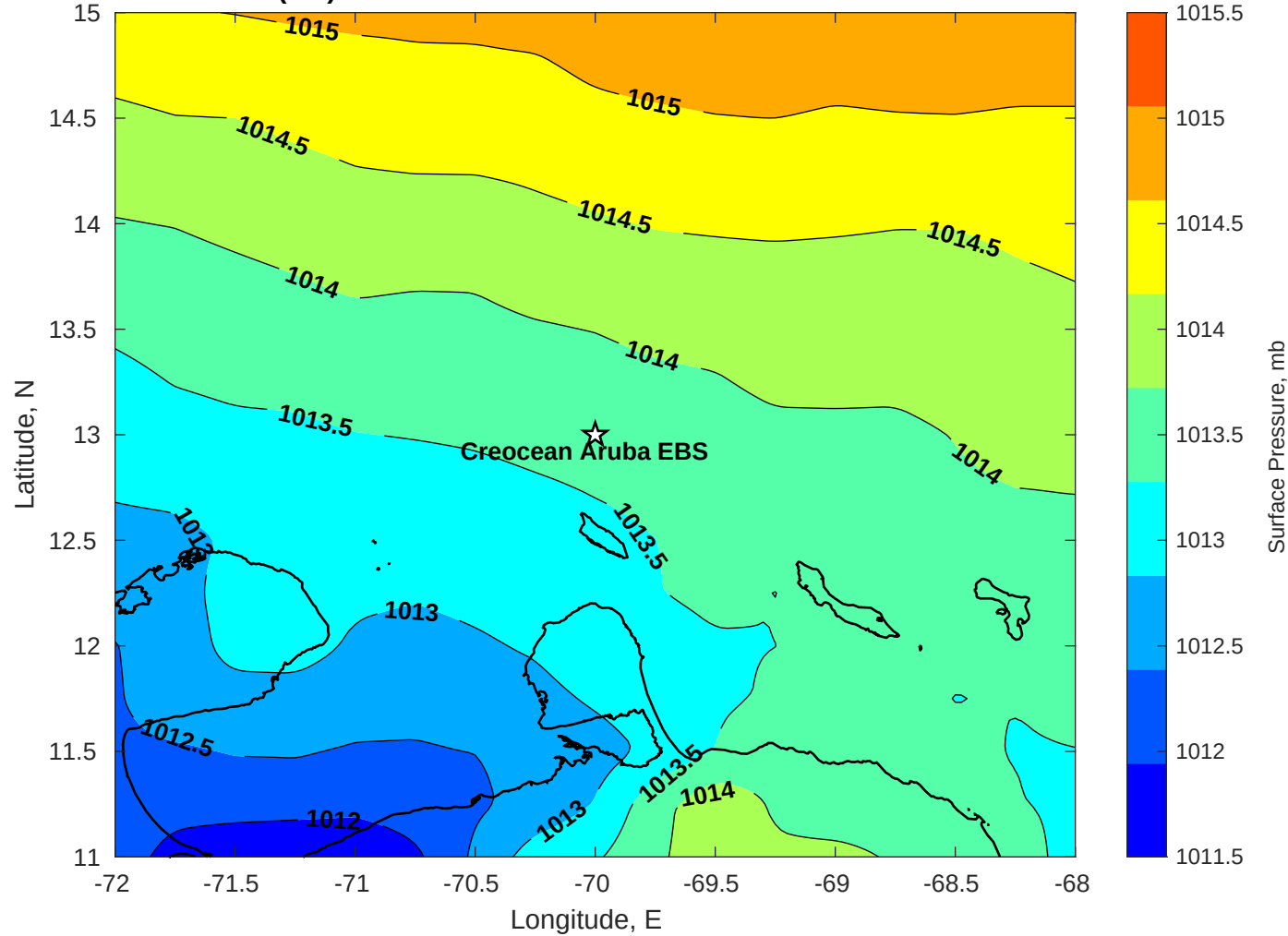
Surface Pressure (mb) for Creoccean Aruba EBS at 26-Jan-2026 06:00:00
