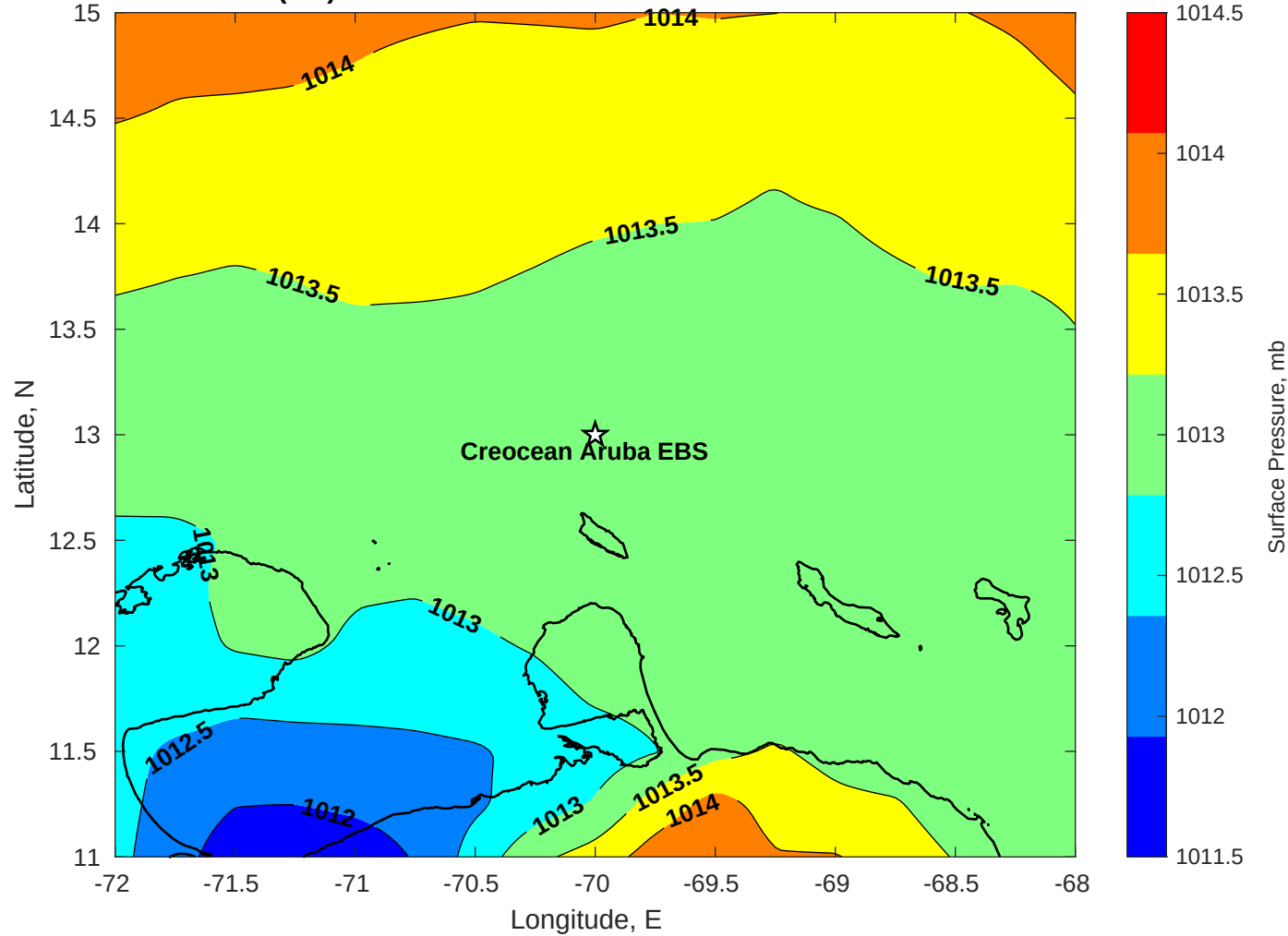
Surface Pressure (mb) for Creoccean Aruba EBS at 28-Jan-2026 06:00:00
