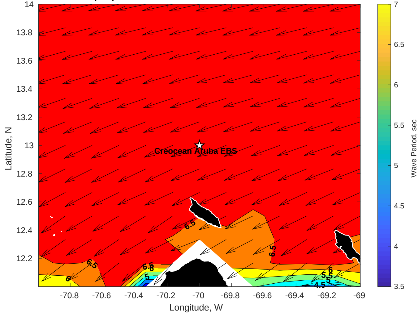
GFS Wave Period (sec) for Creoccean Aruba EBS at 26-Jan-2026 09:00:00
