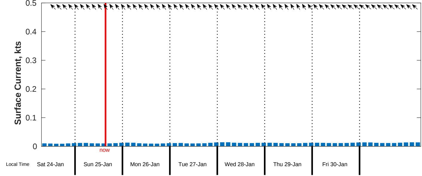
Surface Current Forecast for Creocean Aruba EBS from 25-Jan-2026 00:00:00 to 02-Feb-2026 00:00:00
