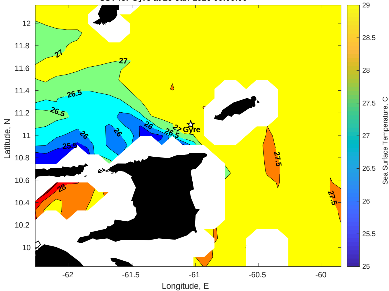
SST for Gyre at 25-Jan-2026 00:00:00
