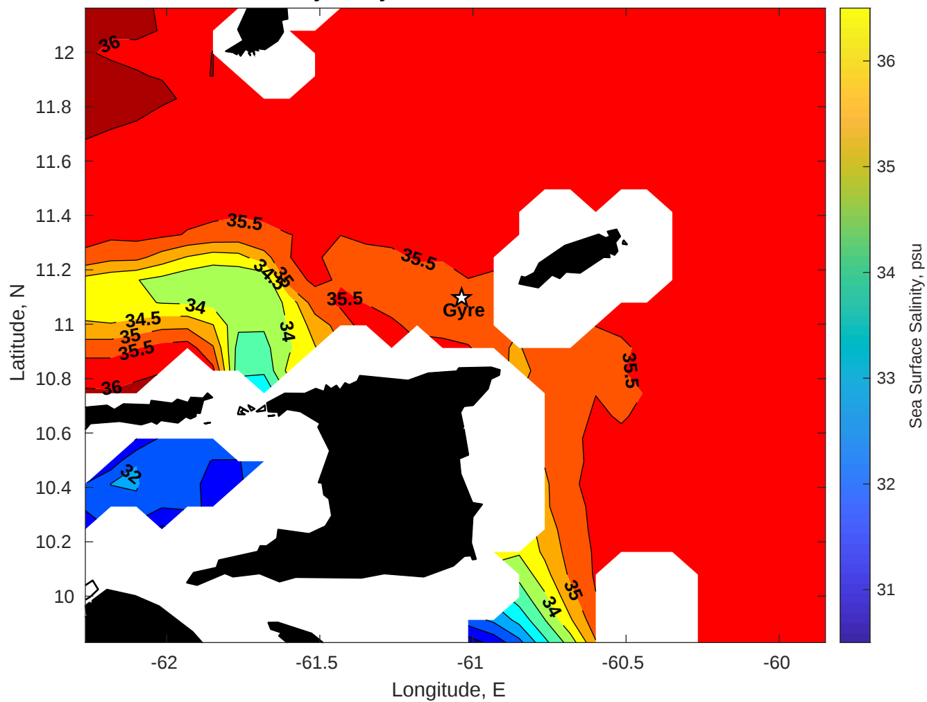
Surface Salinity for Gyre at 25-Jan-2026 00:00:00
