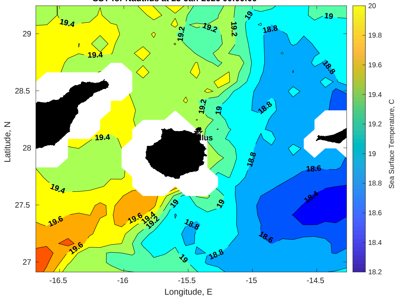
SST for Nautilus at 25-Jan-2026 00:00:00
