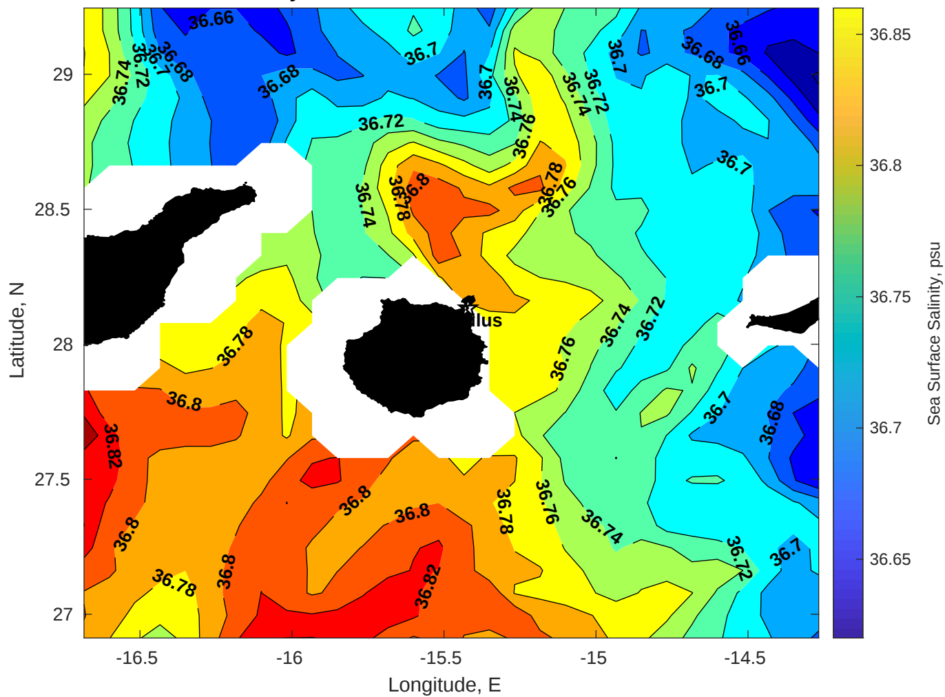
Surface Salinity for Nautilus at 25-Jan-2026 00:00:00
