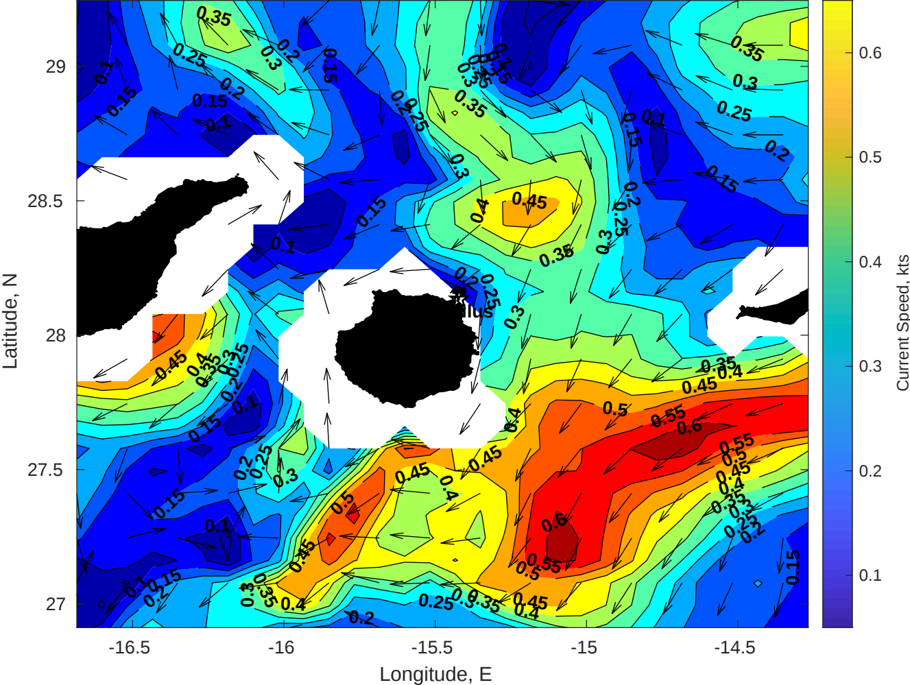
Surface Currents for Nautilus at 25-Jan-2026 00:00:00
